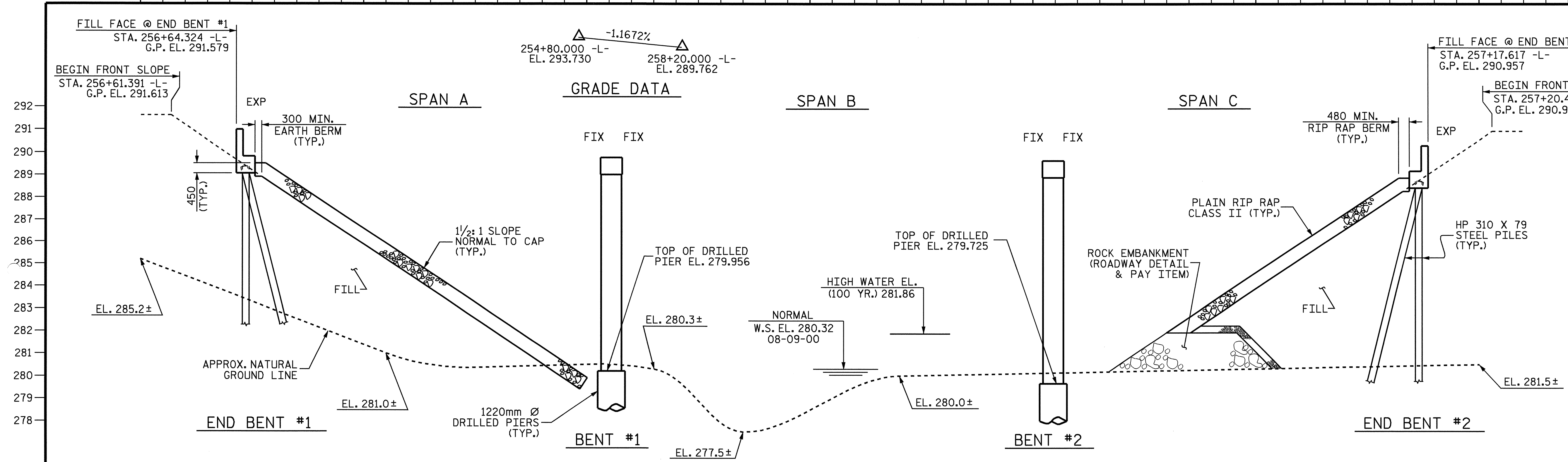
SECTION ALONG GRADE LINE-RIGHT LANE
