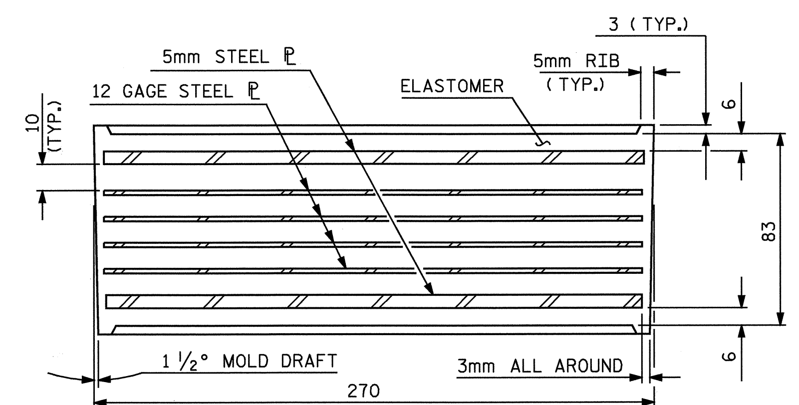
TYPICAL SECTION OF ELASTOMERIC BEARING
