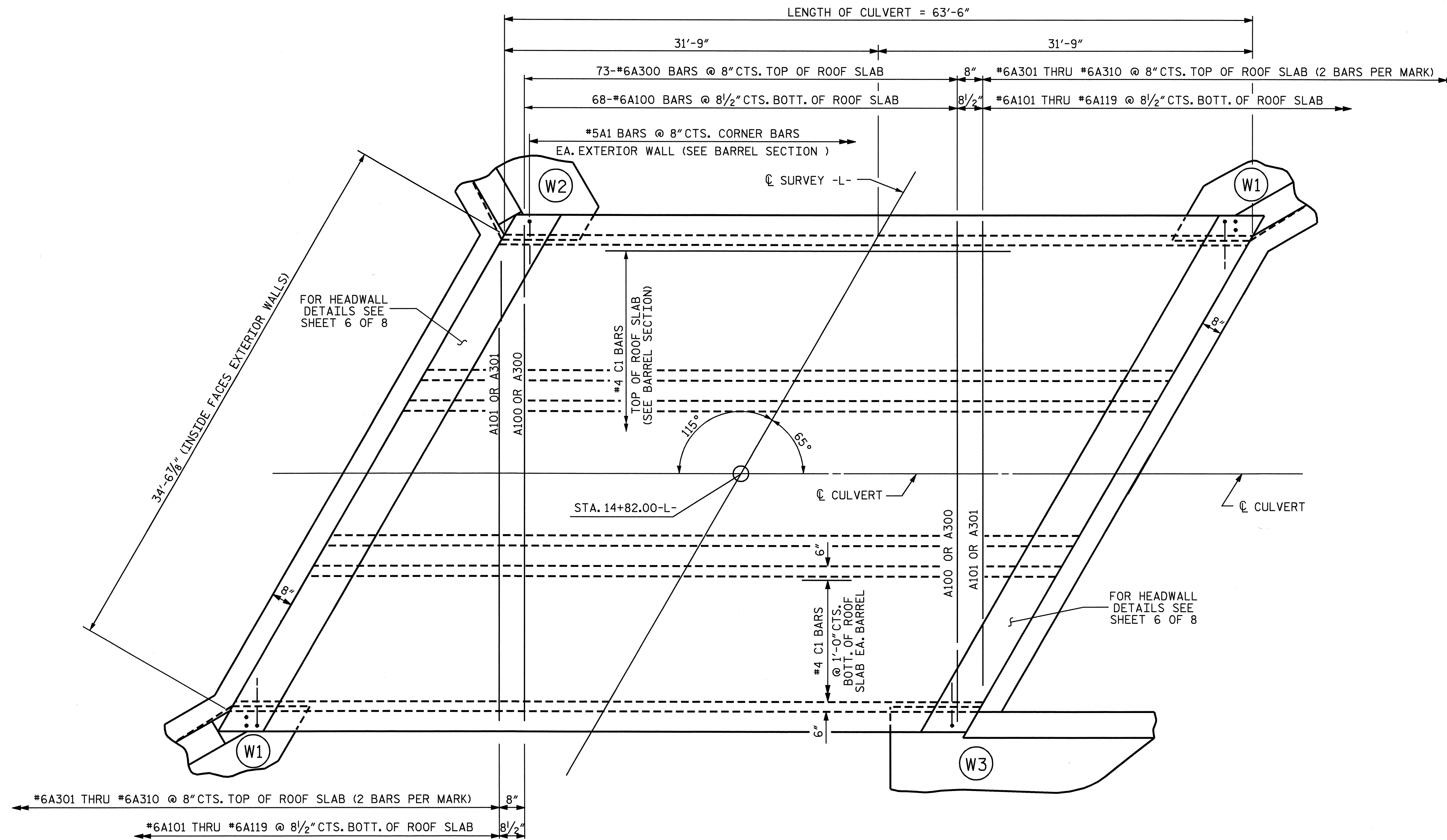
PLAN OF ROOF SLAB
