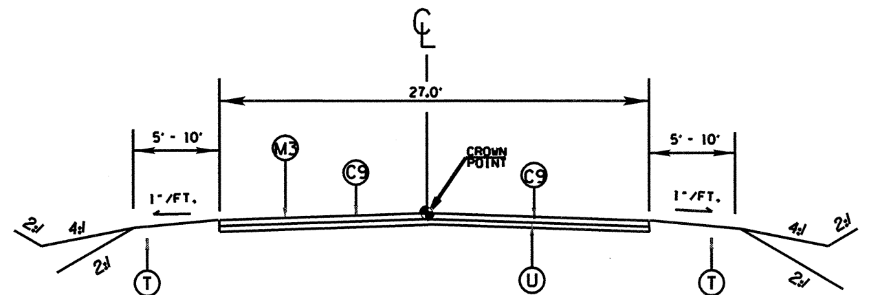
TYPICAL SECTION NO. 14
