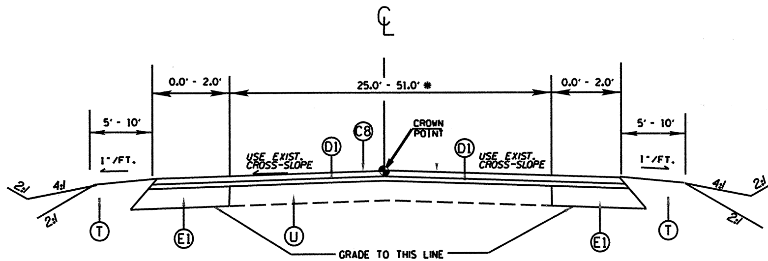
TYPICAL SECTION NO. 12
