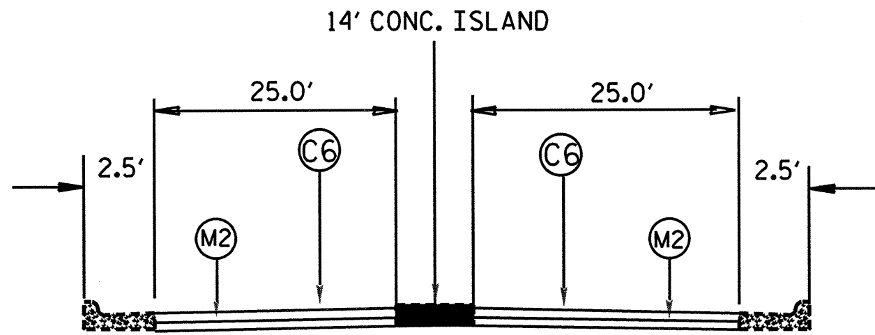
TYPICAL SECTION NO. 11
