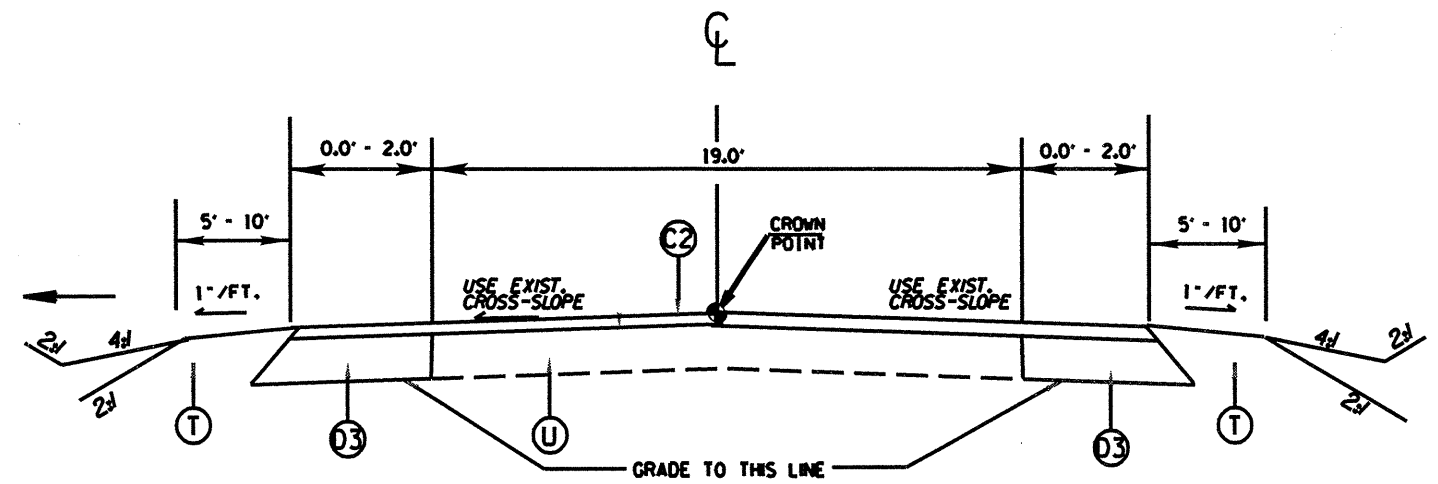
TYPICAL SECTION NO. 22
