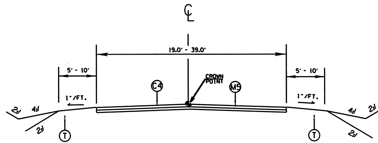
TYPICAL SECTION NO. 20
