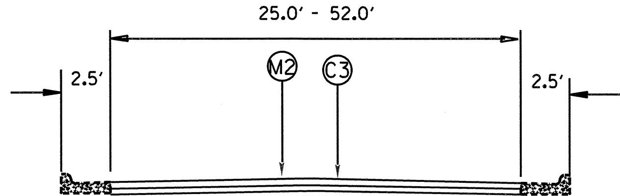
TYPICAL SECTION NO. 21
