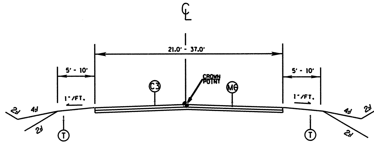
TYPICAL SECTION NO. 19
