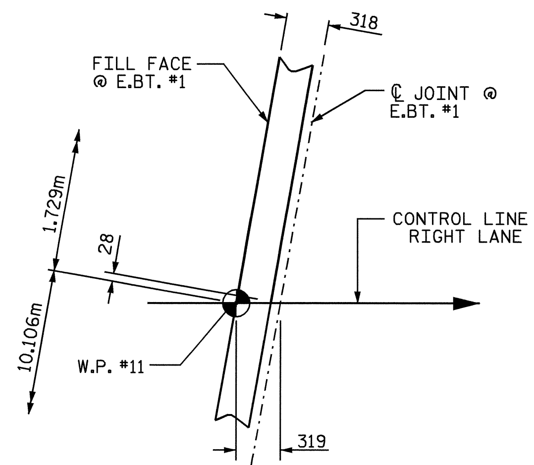
DETAIL A
