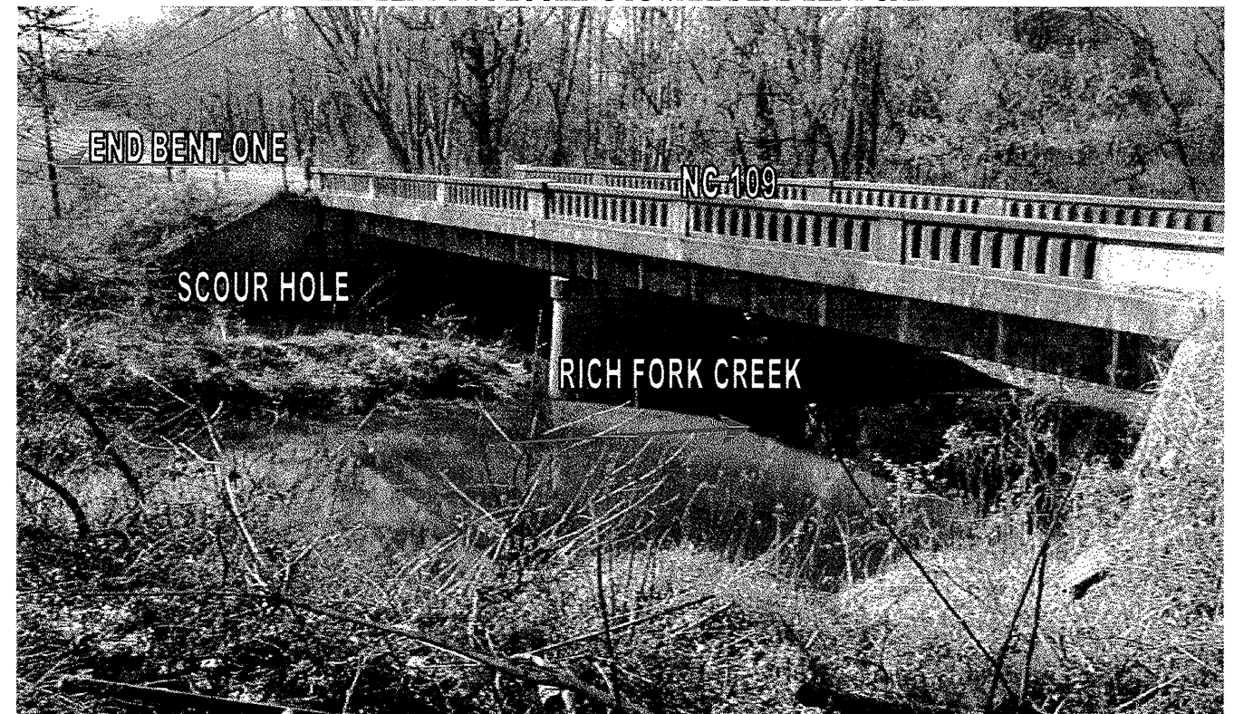
END BENT TWO LOOKING TOWARDS END BENT ONE
