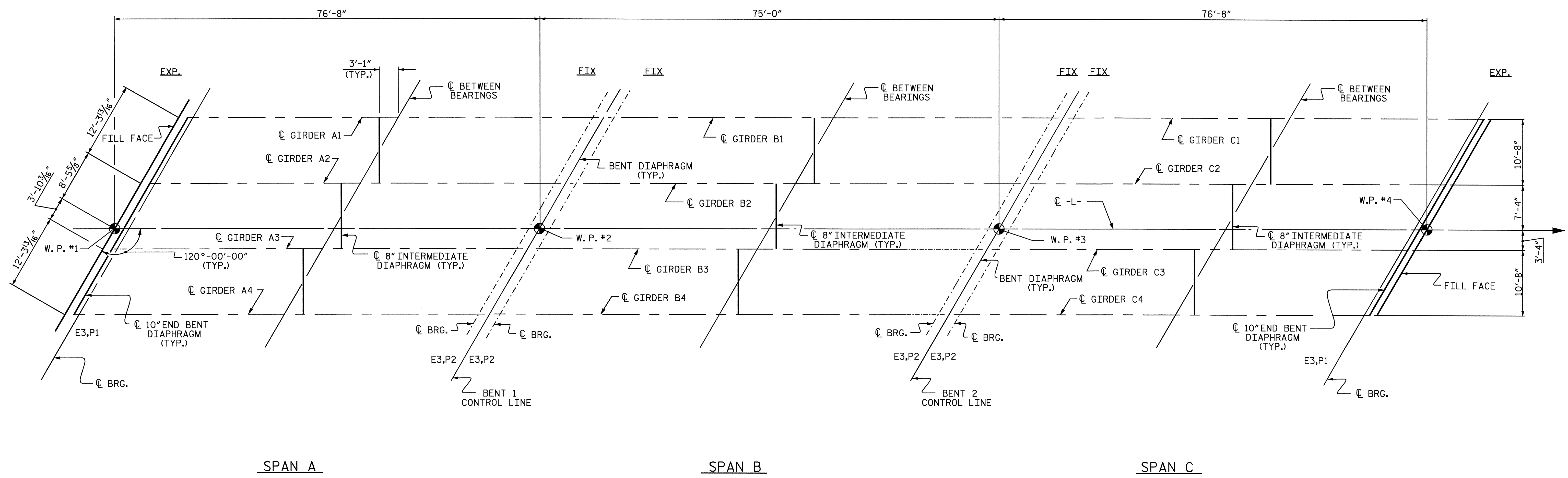
PLAN OF GIRDER LAYOUT
