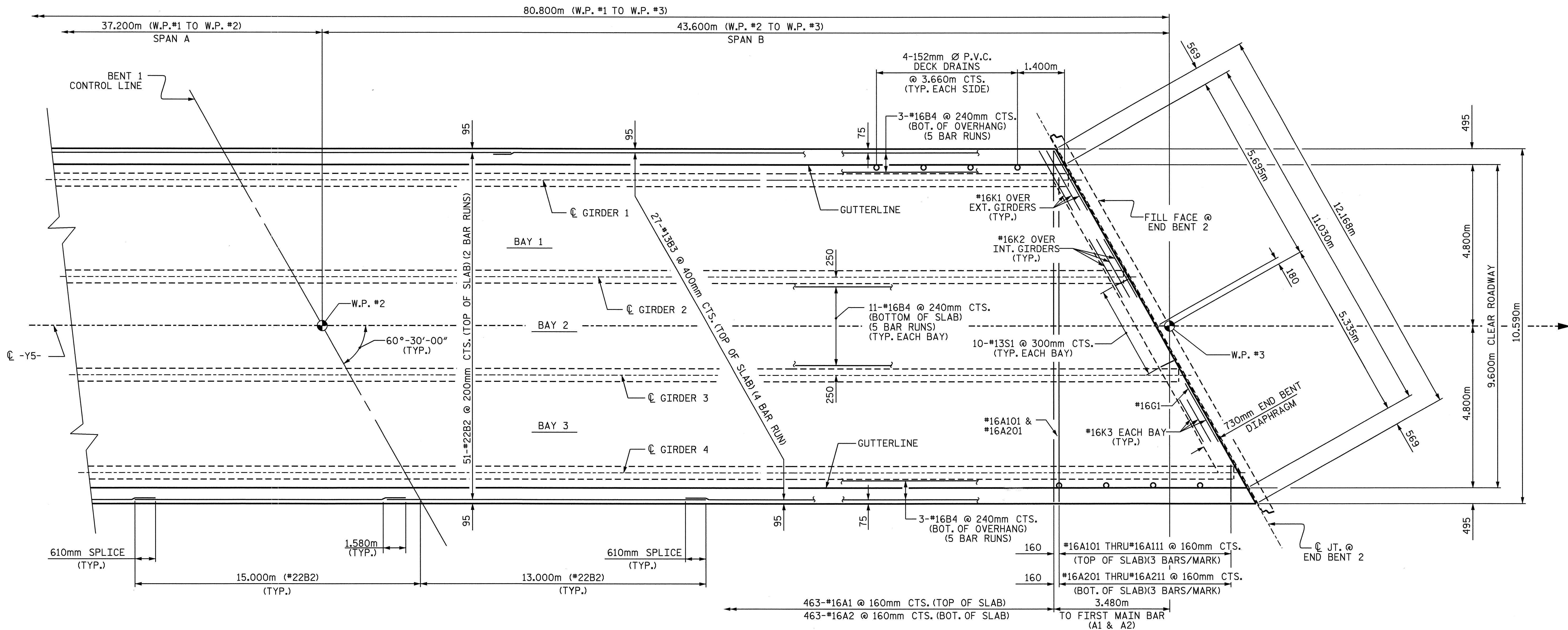
PLAN OF SPAN B BARRIER RAIL NOT SHOWN FOR CLARITY.
