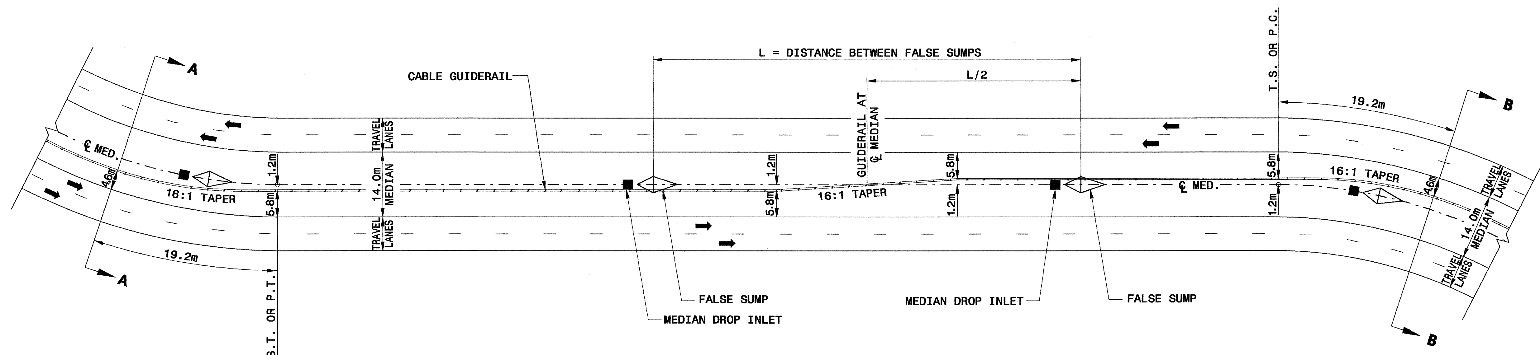
PLAN VIEW
