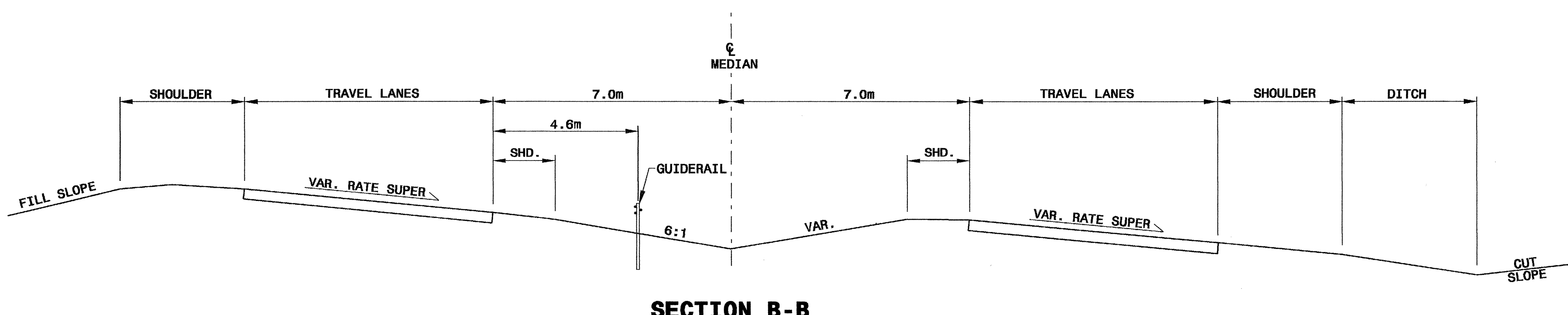
SECTION B-B
