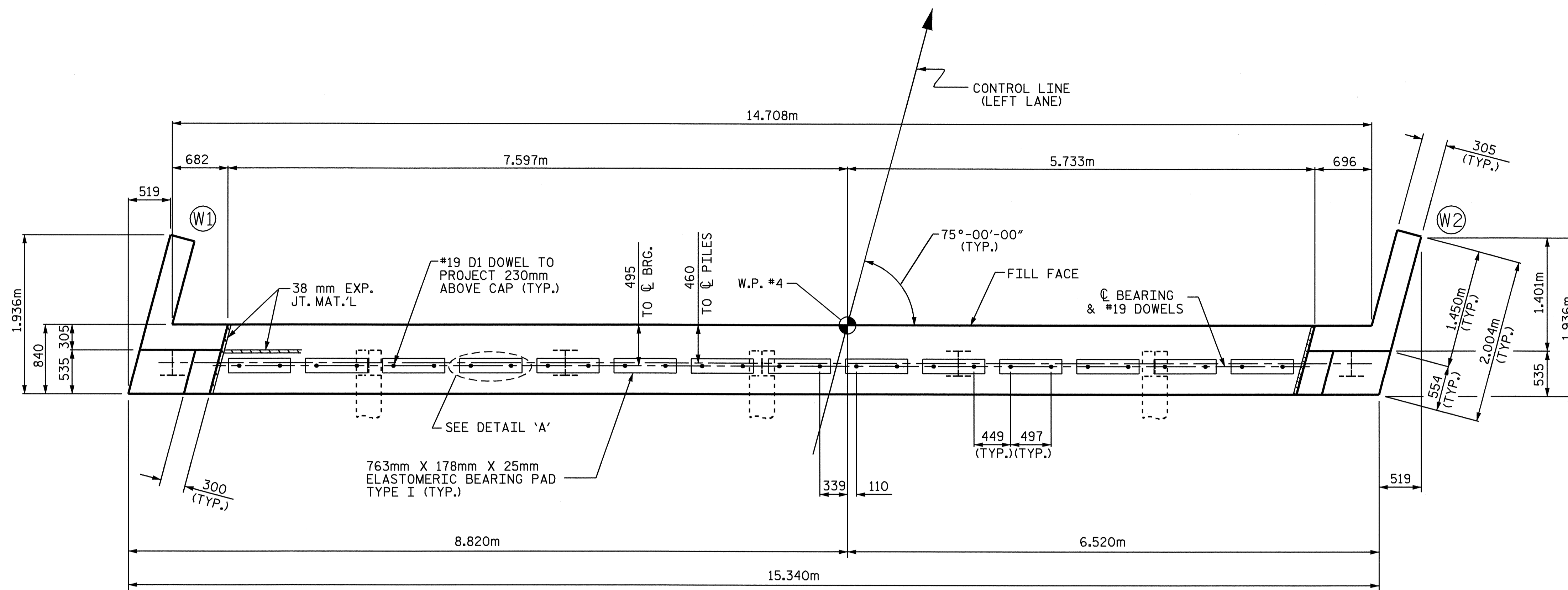
PLAN
