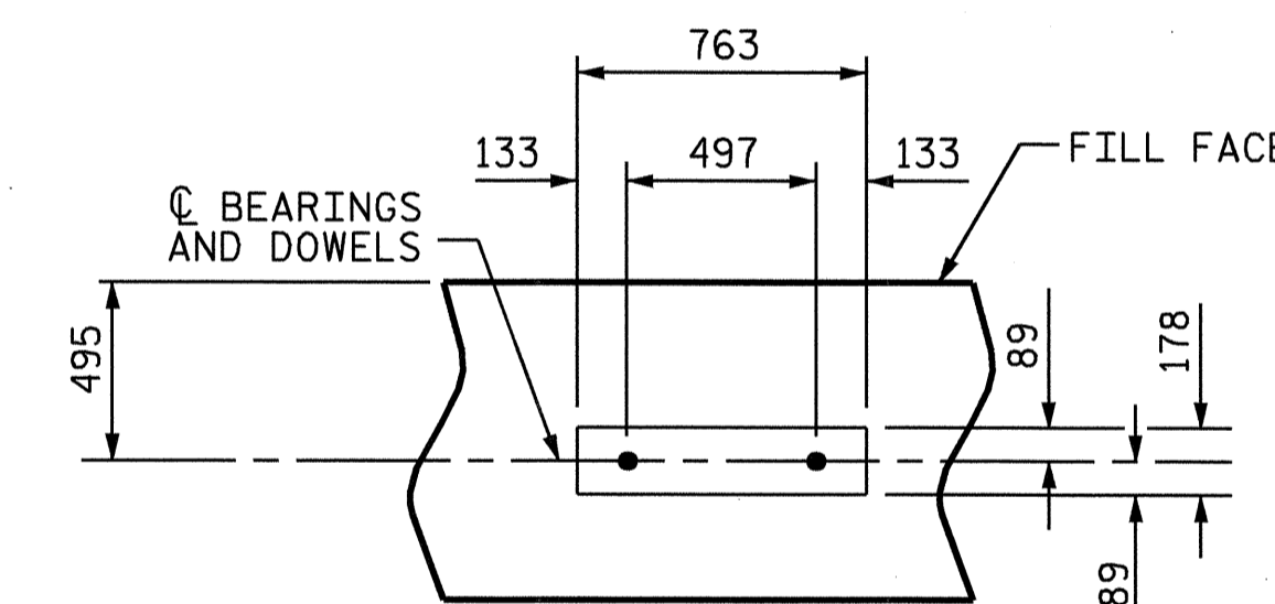
DETAIL "A"
