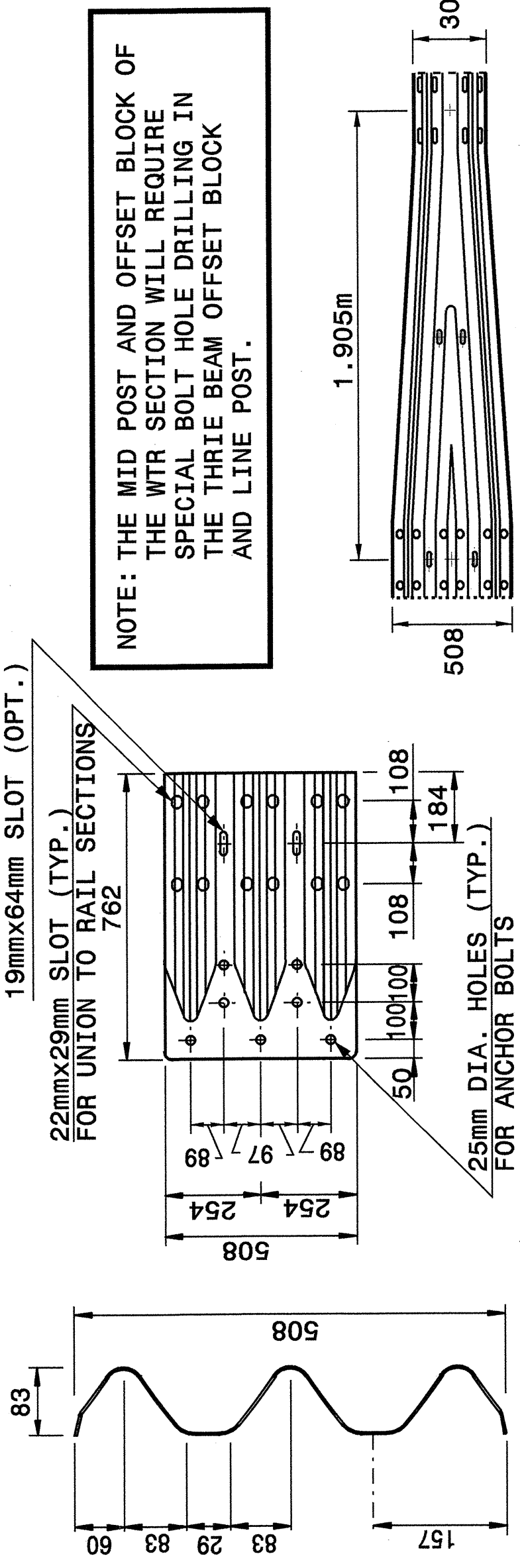
WTR SECTION ELEVATION VIEW
