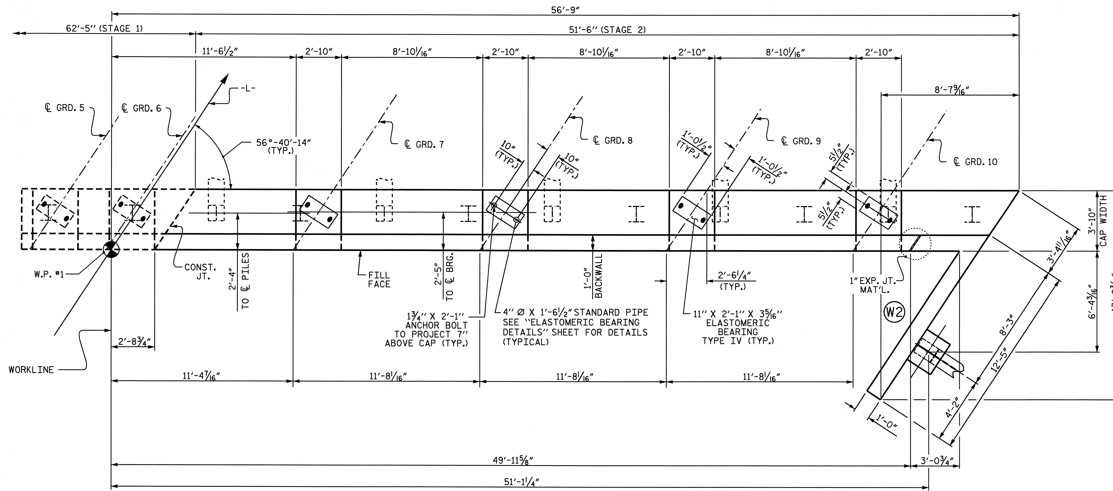
PLAN
