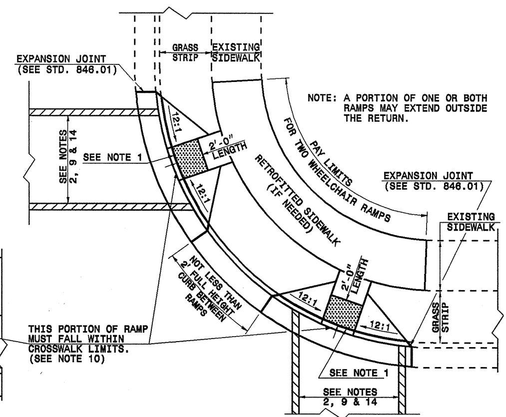
PLAN VIEW DUAL RAMP ANY RADII (40" MIN. FLOOR WIDTH)
