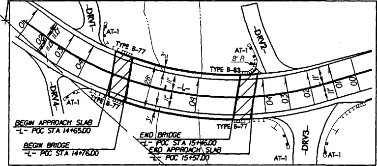
SKETCH OF BRIDGE IN RELATIONSHIP TO PAVEMENT
