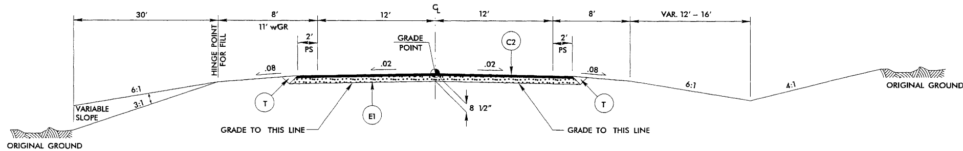
TYPICAL ROADWAY SECTION 2
