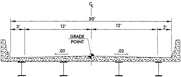
TYPICAL SECTION ON STRUCTURE
