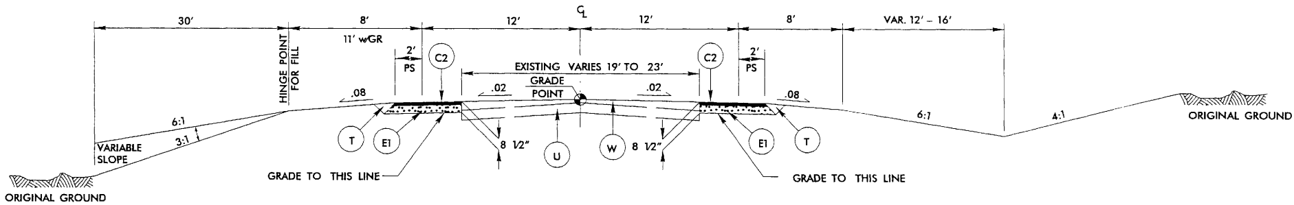
TYPICAL ROADWAY SECTION 1
