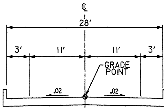
BRIDGE TYPICAL SECTION
