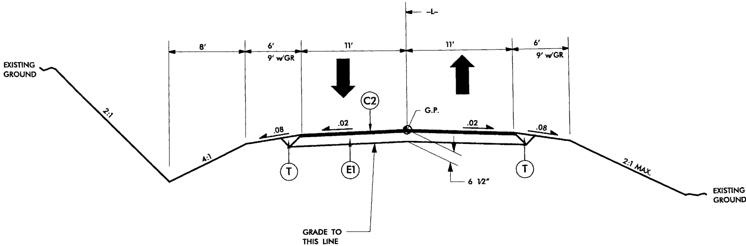
TYPICAL SECTION NO. 2 -L- STA 18+00 TO -L- STA 18+32.02 (APPROACH SLAB) -L- STA 19+74.98.00 (APPROACH SLAB) TO -L- STA 20+00
