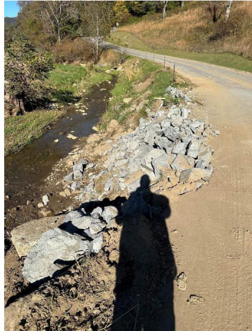
Figure 6. Damage to Culvert 449 from Hurricane Helene. North side of culvert, looking north-northeast. Note debris has been removed and temporary road repair has occurred. NCDOT Hurricane Helene All Imagery/Drone Map, December 30, 2024.
