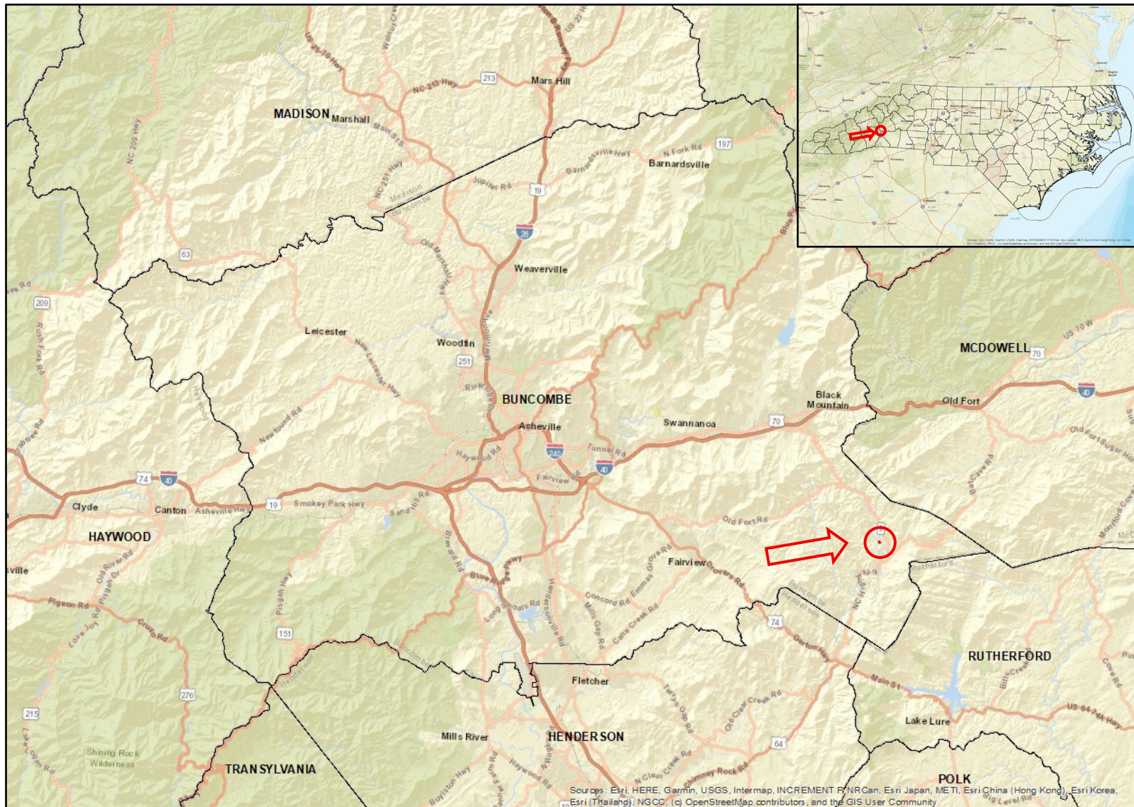
Figure 1: Location of the study area in Buncombe County, North Carolina.
