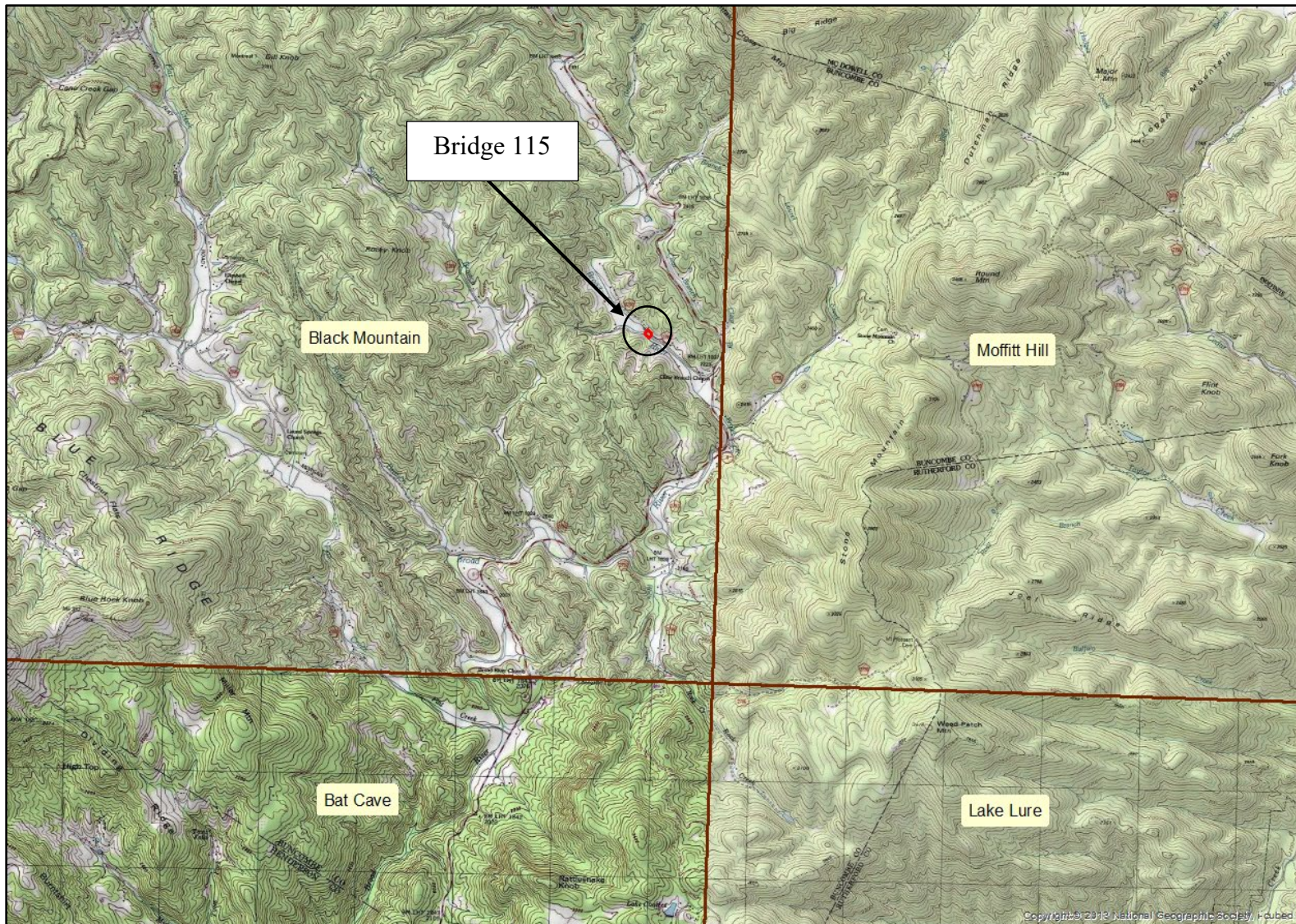
Figure 2: Location of the study area on the USGS Black Mountain , Moffitt Hill , Bat Cave and Lake Lure topographic maps.
