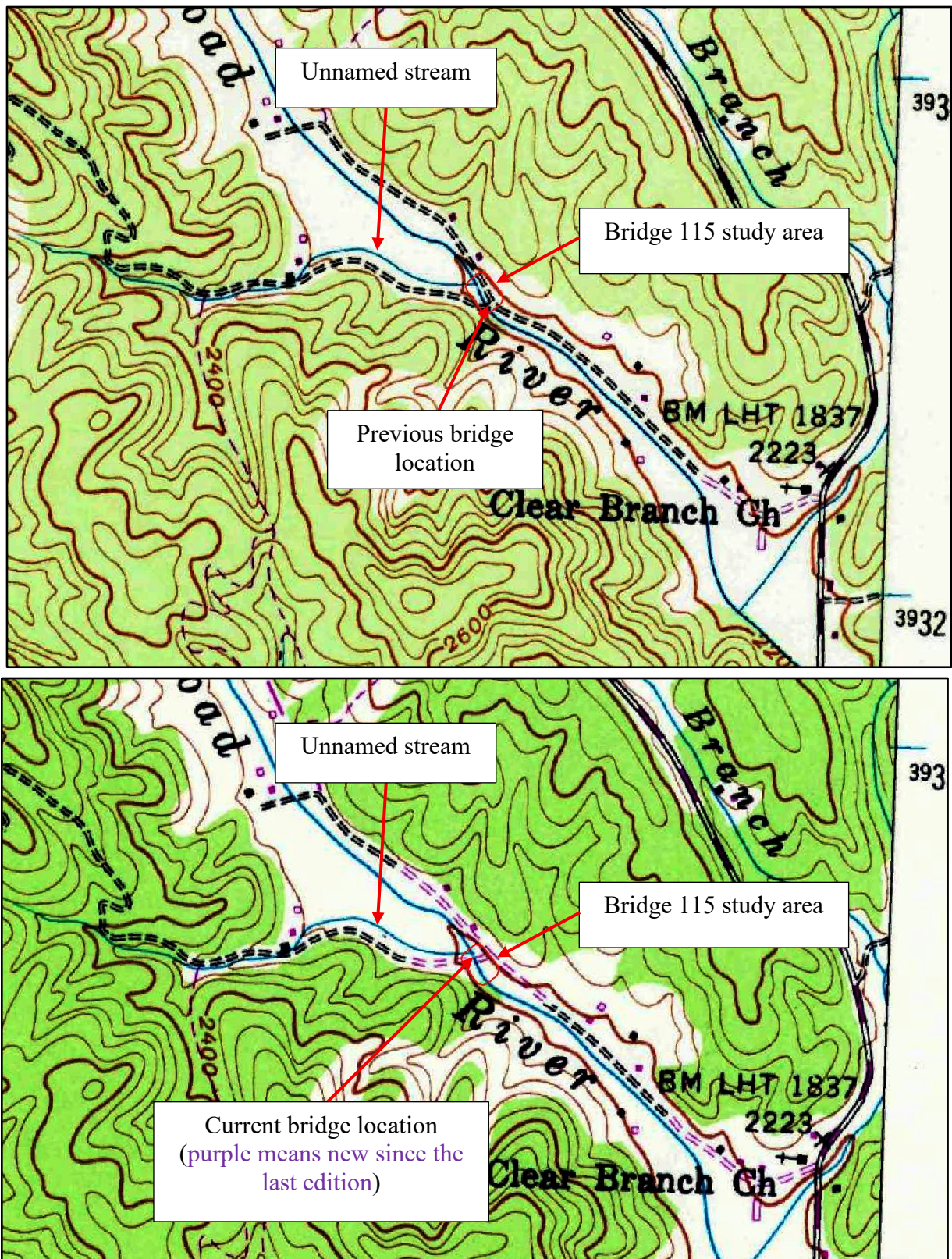
Figure 4: Topographic maps of the study area in 1969 (top) and 1978 (bottom) (USGS 1969 and 1978 Black Mountain 1:24,000-scale topographic maps).
