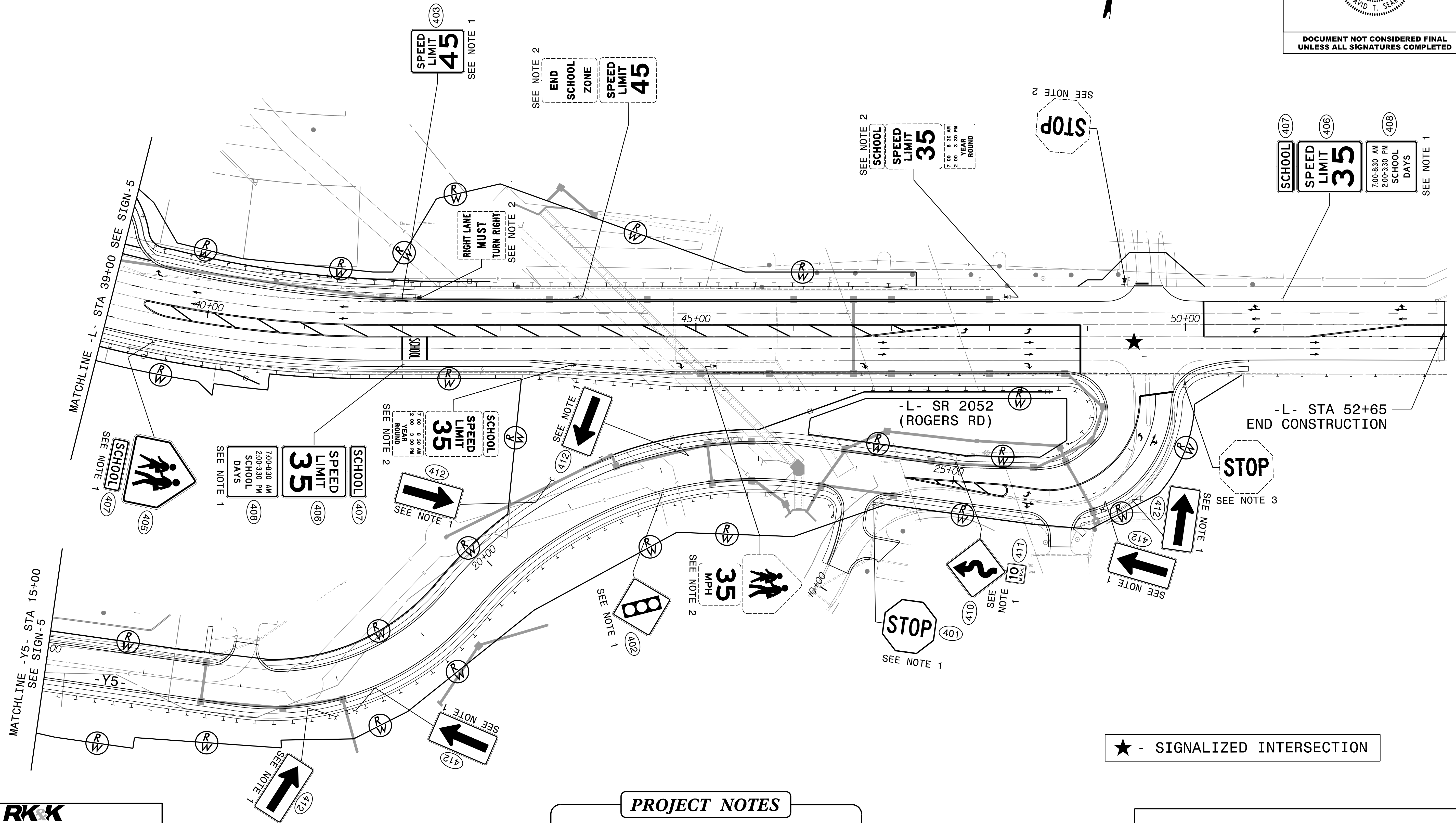
SIGNING PLAN
