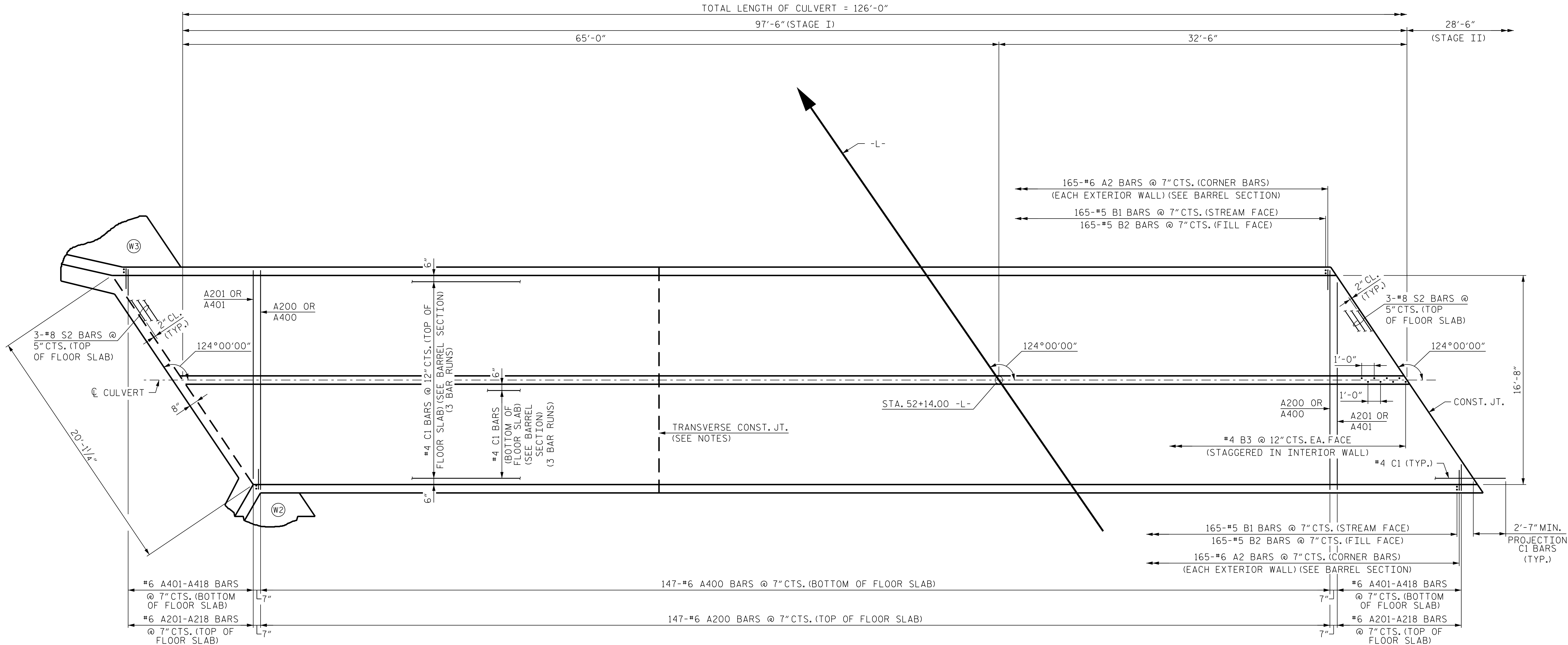
PLAN - FLOOR SLAB STAGE I
