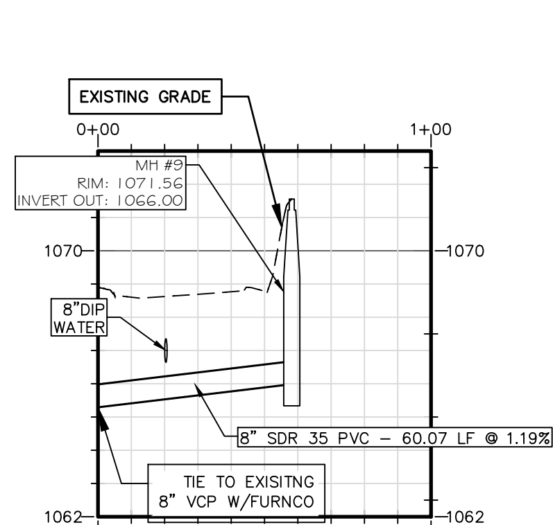
SEWER 7
