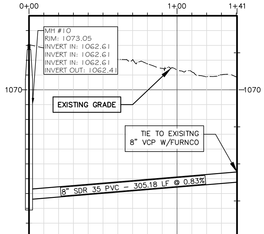
SEWER 8
