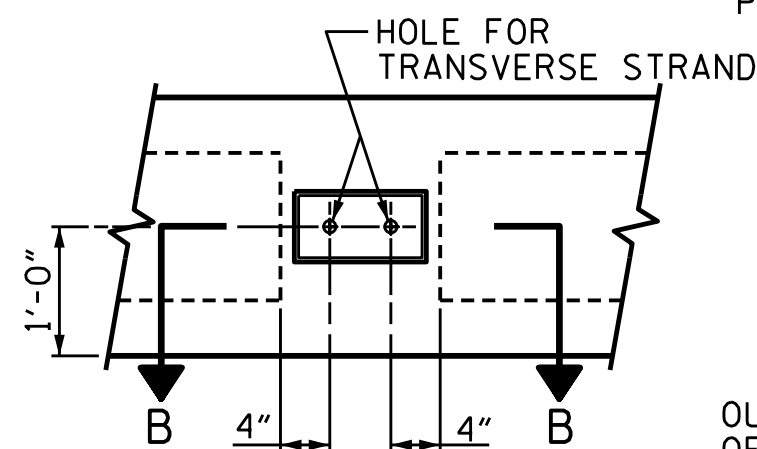
ELEVATION VIEW
