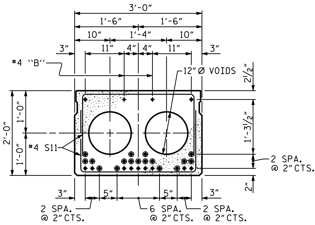
INTERIOR SLAB SECTION (35' UNIT) (11 STRANDS REQUIRED)
