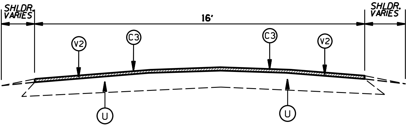
TYPICAL SECTION NO. 21
