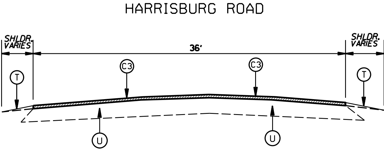
TYPICAL SECTION NO. 20
