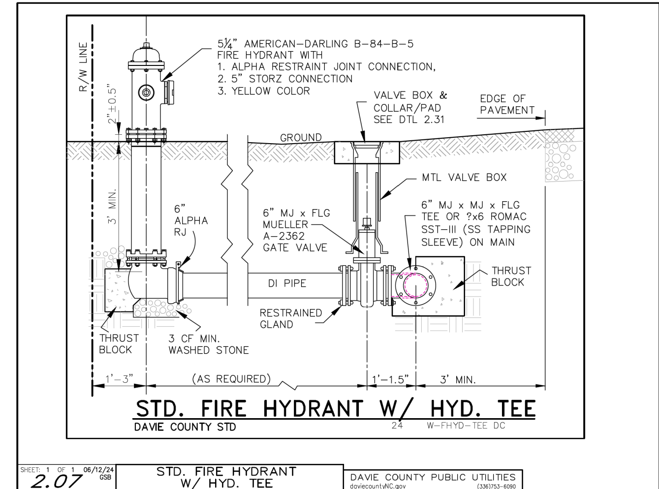
2.07 STD. FIRE HYDRANT W/ HYD. TEE DAVE COUNTY PUBLIC UTILITIES
