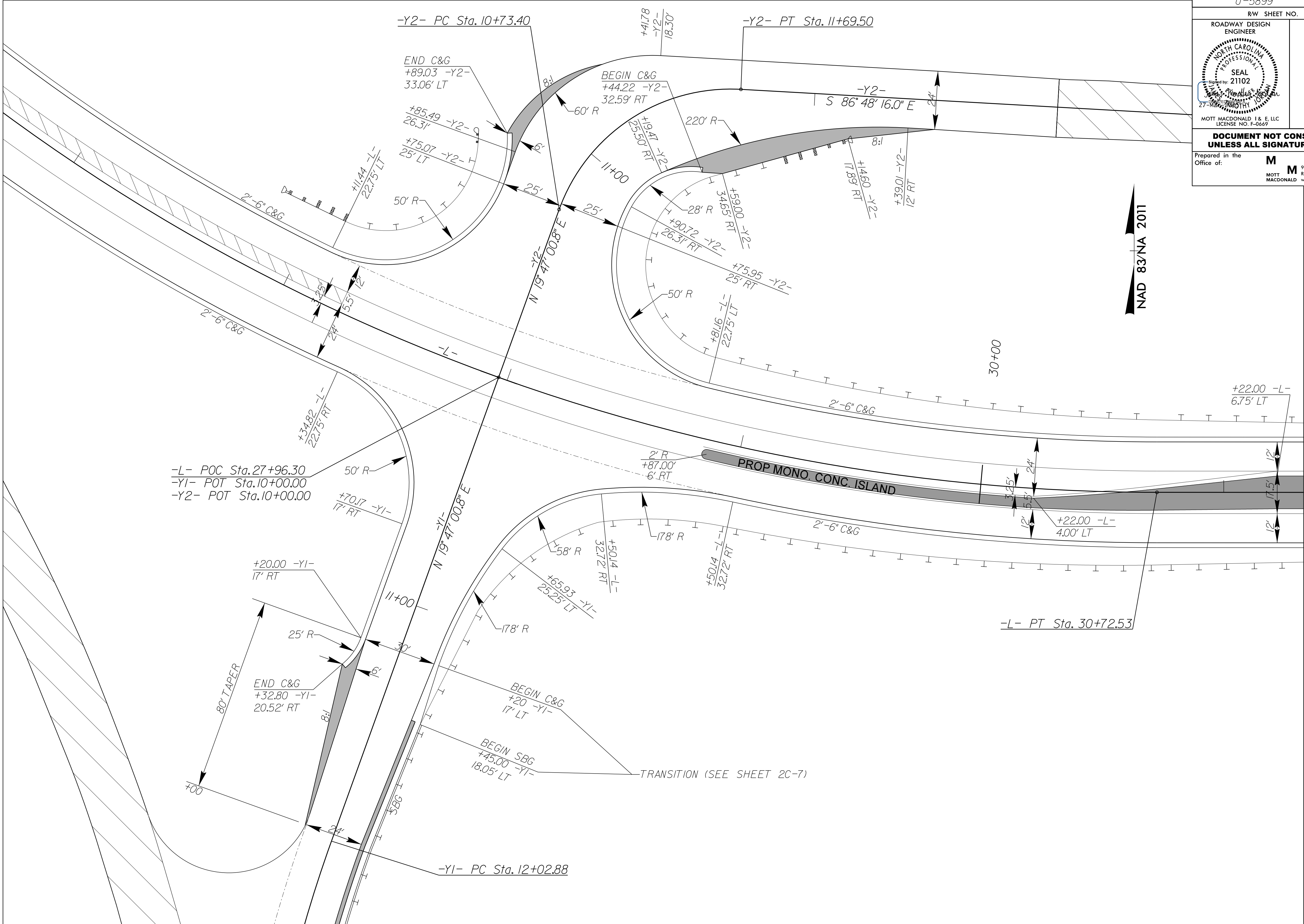
INTERSECTION DETAIL -L- /-Y1- /-Y2- FOR PLAN SEE SHEET 5
