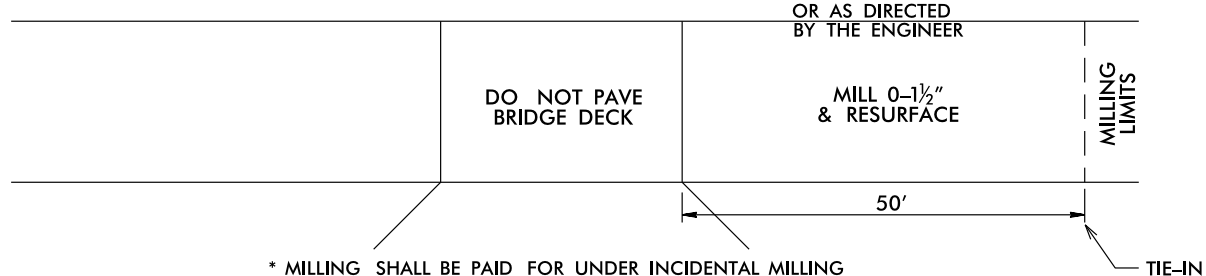
* MILLING SHALL BE PAID FOR UNDER INCIDENTAL MILLING DRAWING FOR MAP 5 SR 2114 PROVIDENCE CHURCH RD BRIDGE #108
