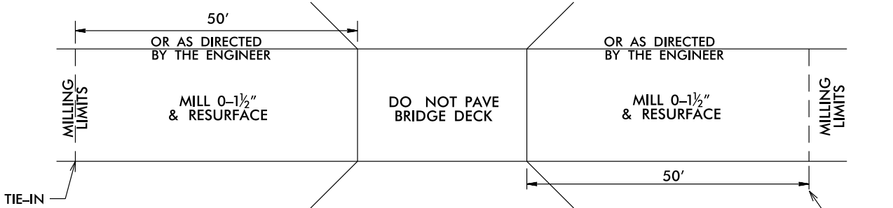
* MILLING SHALL BE PAID FOR UNDER INCIDENTAL MILLING DRAWING FOR MAP 4 SR 2116 NEW SALEM RD BRIDGE #111
