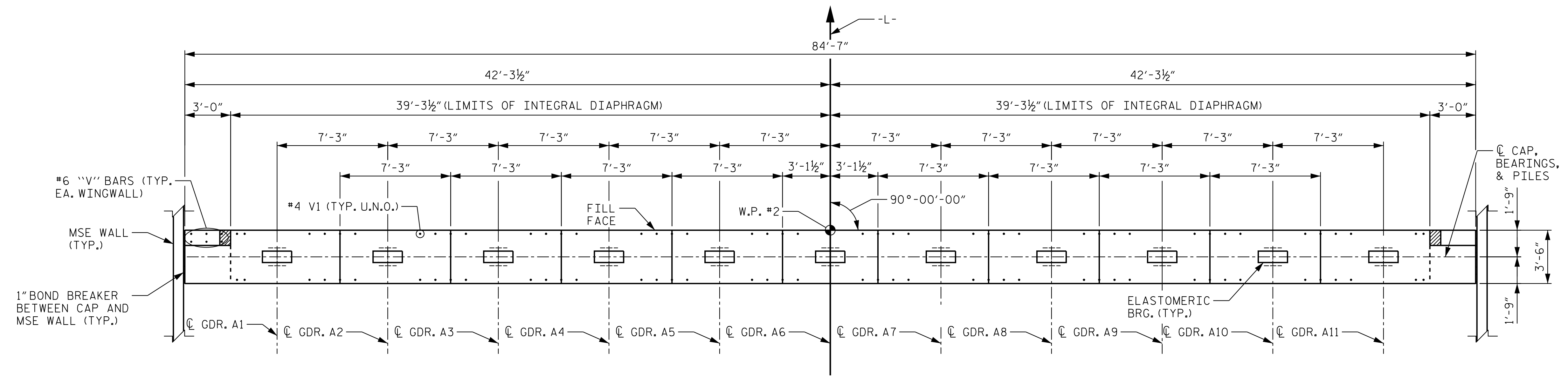
PLAN
