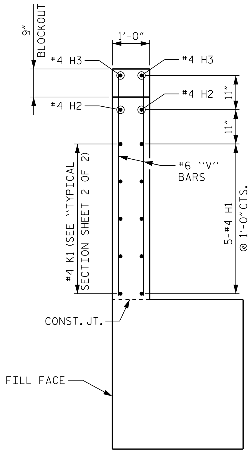
SECTION Y-Y
