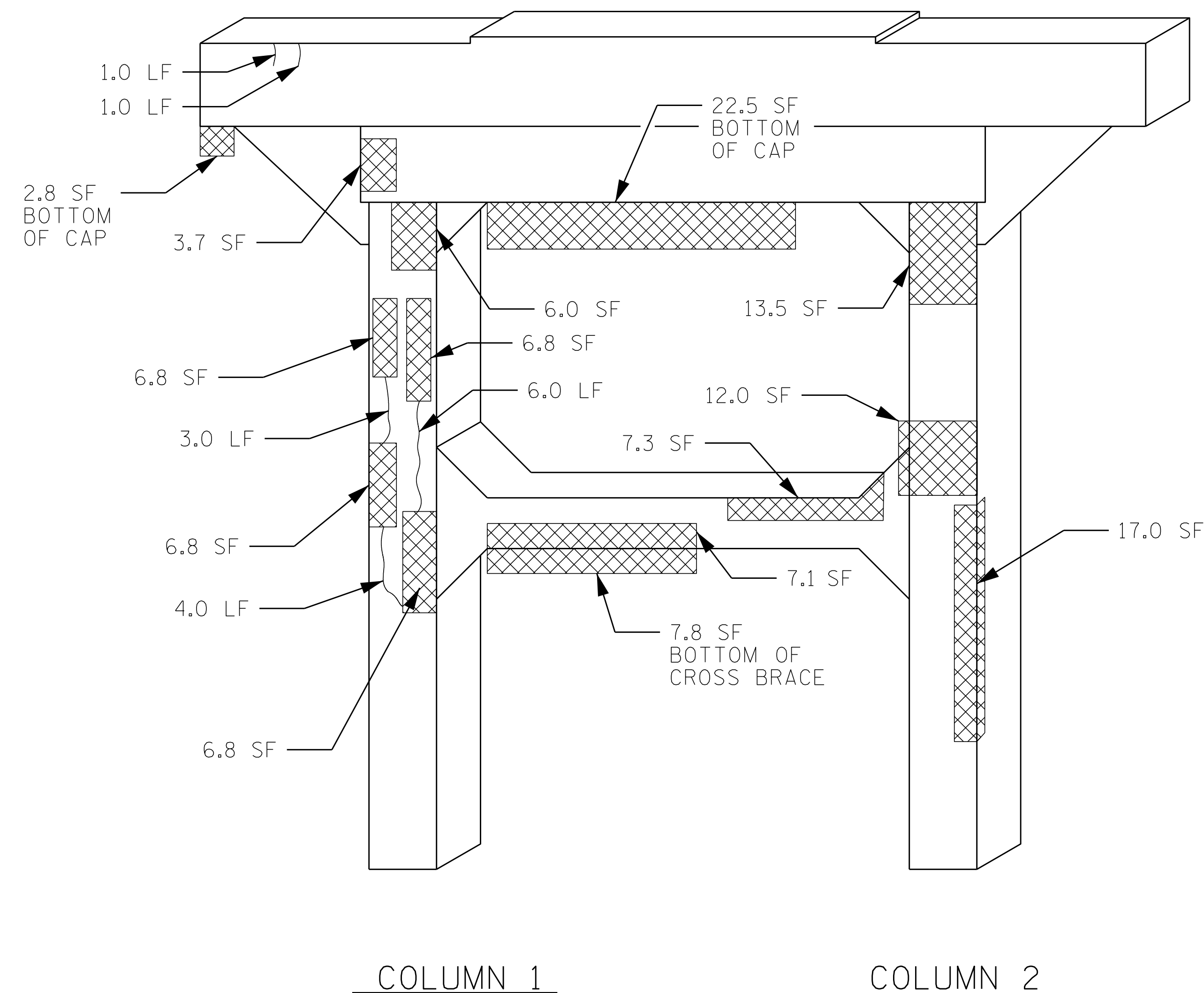
ELEVATION @ BENT 6 (SPAN F)
