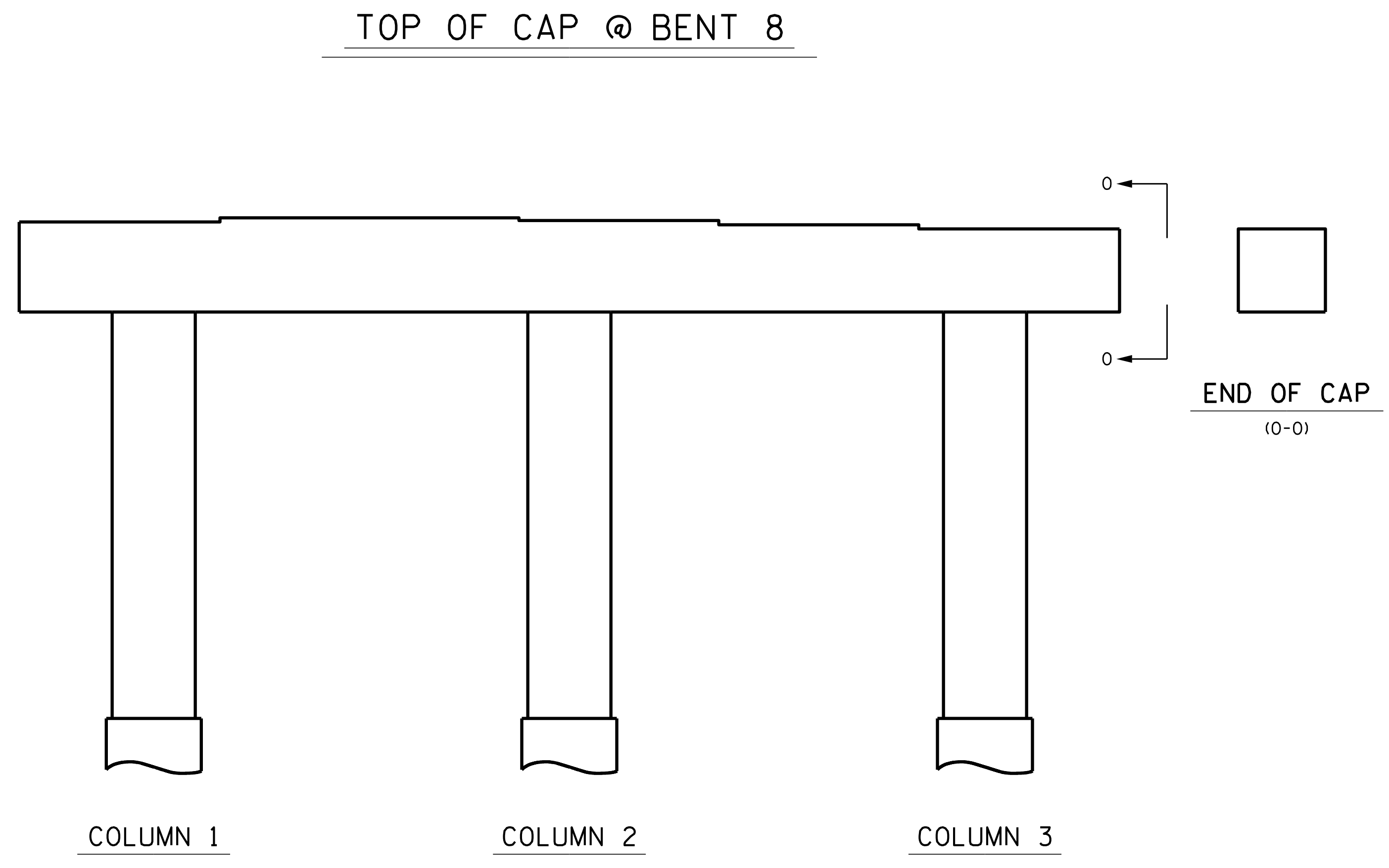
ELEVATION @ BENT 8 (SPAN H)
