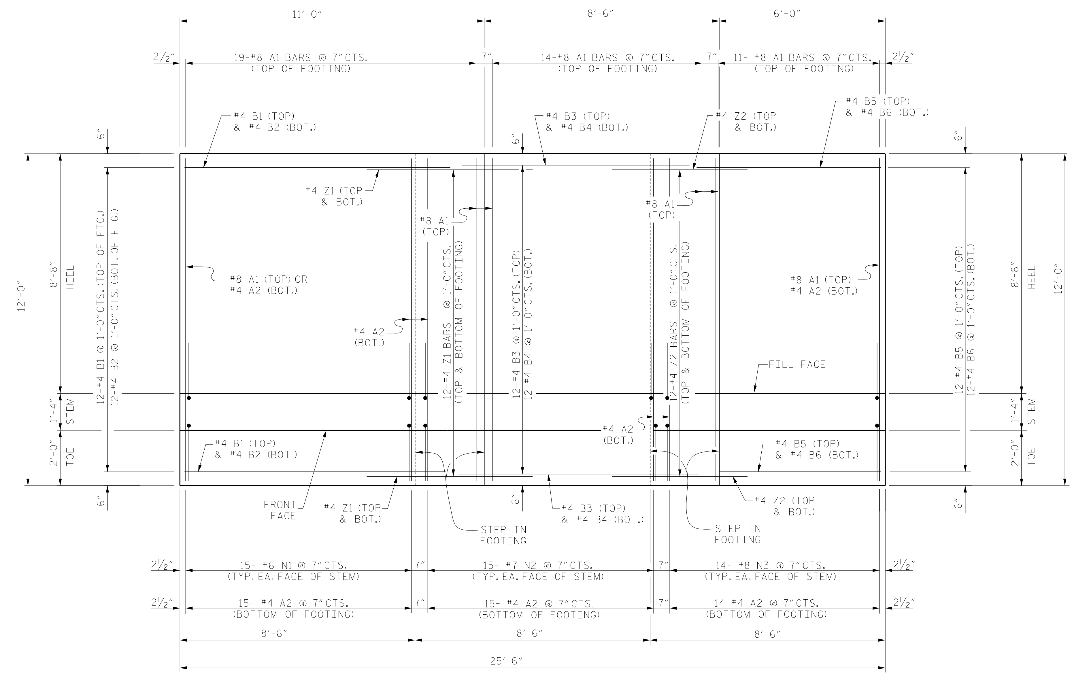
PLAN OF FOOTING
