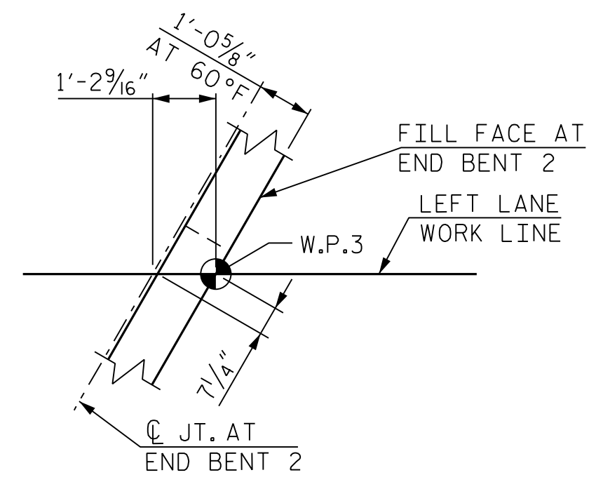
DETAIL "B"
