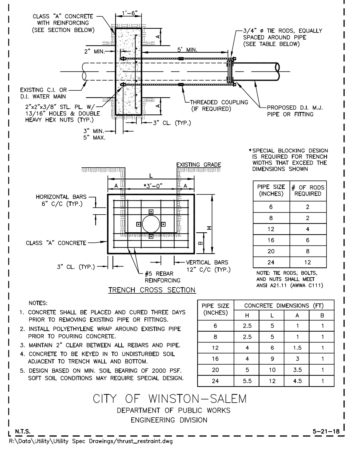
THRUST HARNESS FOR EXISTING PIPE
