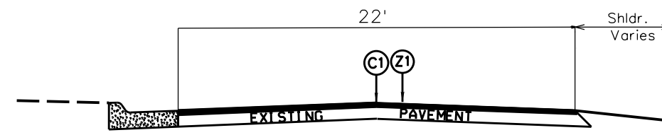
TYPICAL SECTION NO. 8
