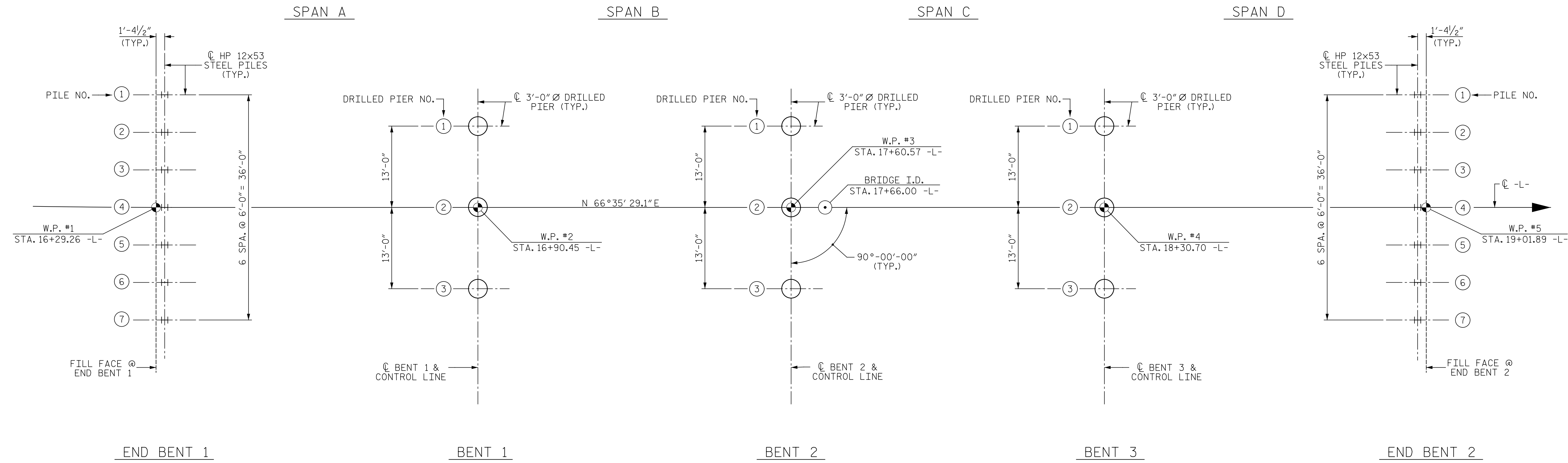
FOUNDATION LAYOUT (PILES DIMENSIONED FROM W.P. TO \phi PILE AT BOT. OF CAP)
