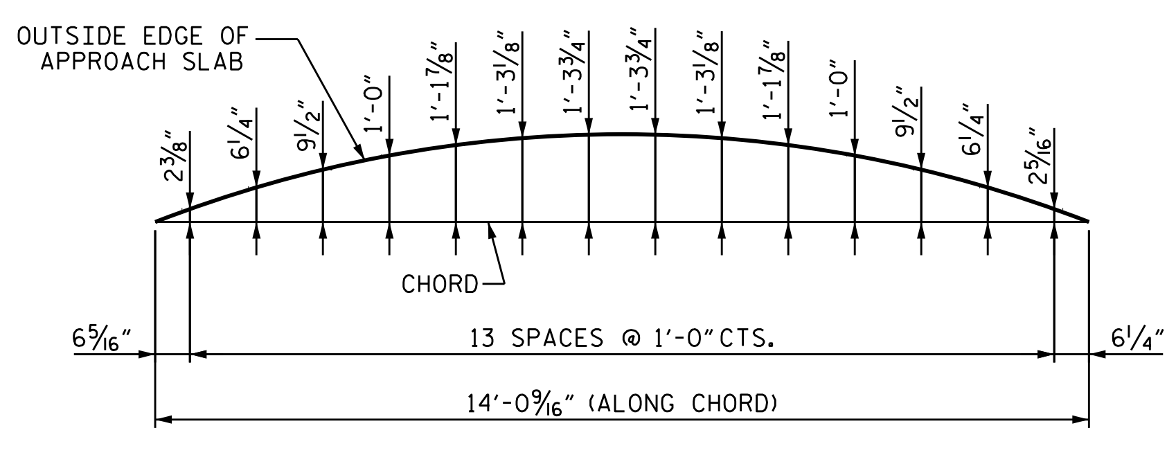
PLAN OF APPROACH SLAB @ END BENT 2
