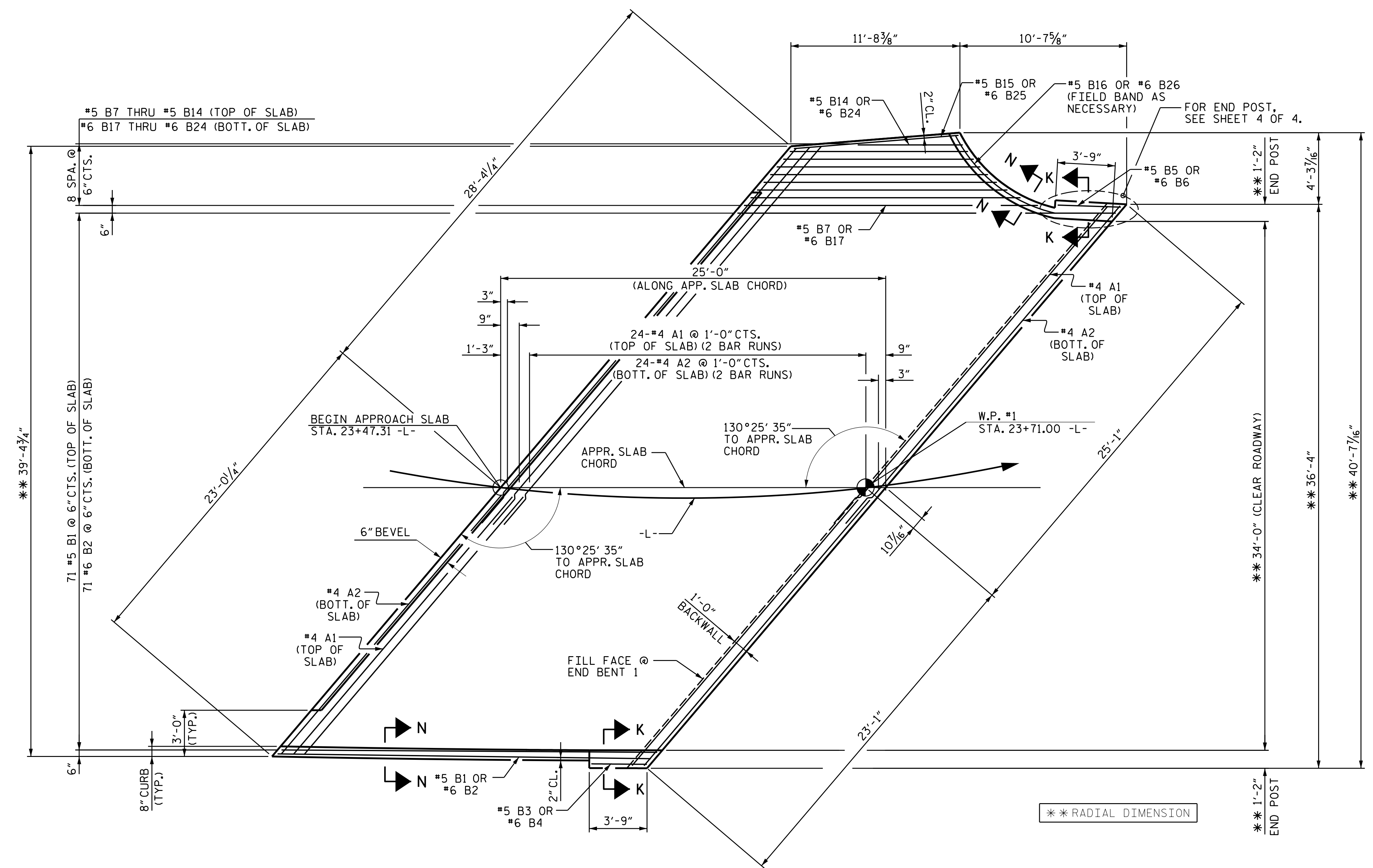
PLAN OF APPROACH SLAB @ END BENT 1
