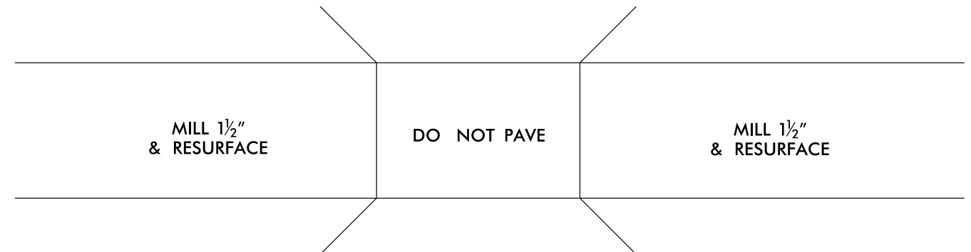
BRIDGE DRAWING FOR MAP #2 US 74 BUS (BRIDGE #75)
