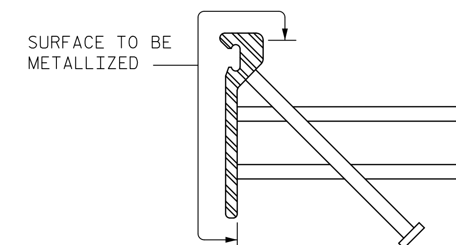
METALLIZING DETAIL
