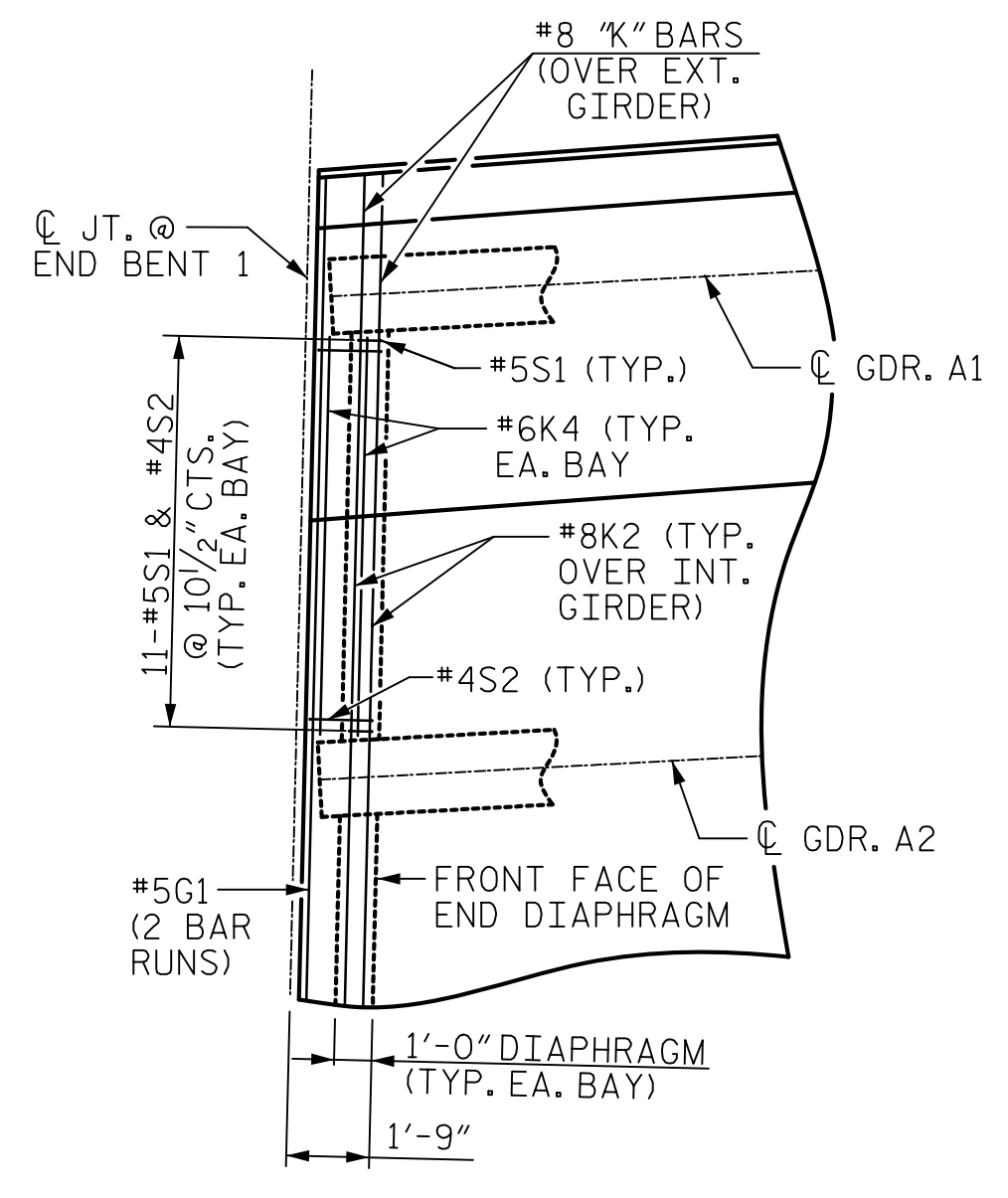
DETAIL "B"
