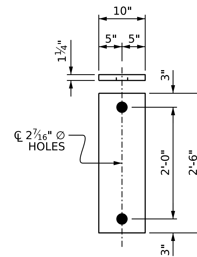
P1 (FIXED)
