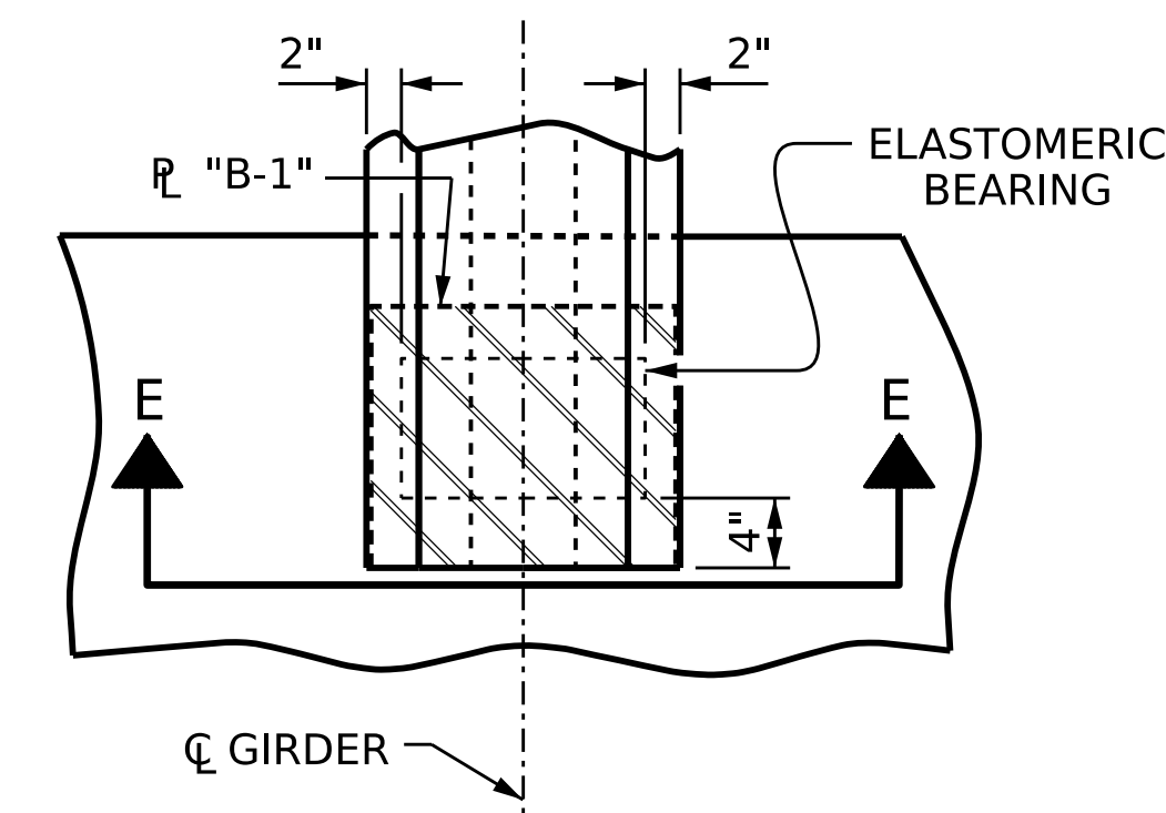
TYPICAL PART PLAN (SHOWING INTEGRAL END BENT)
