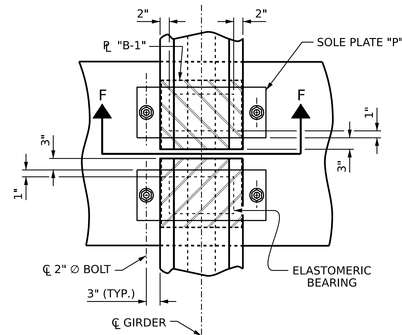
TYPICAL PART PLAN (SHOWING INTERIOR BENT)
