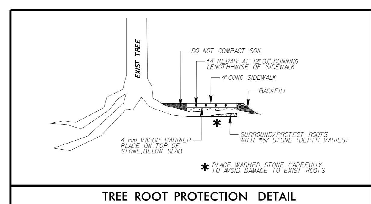
TREE ROOT PROTECTION DETAIL
