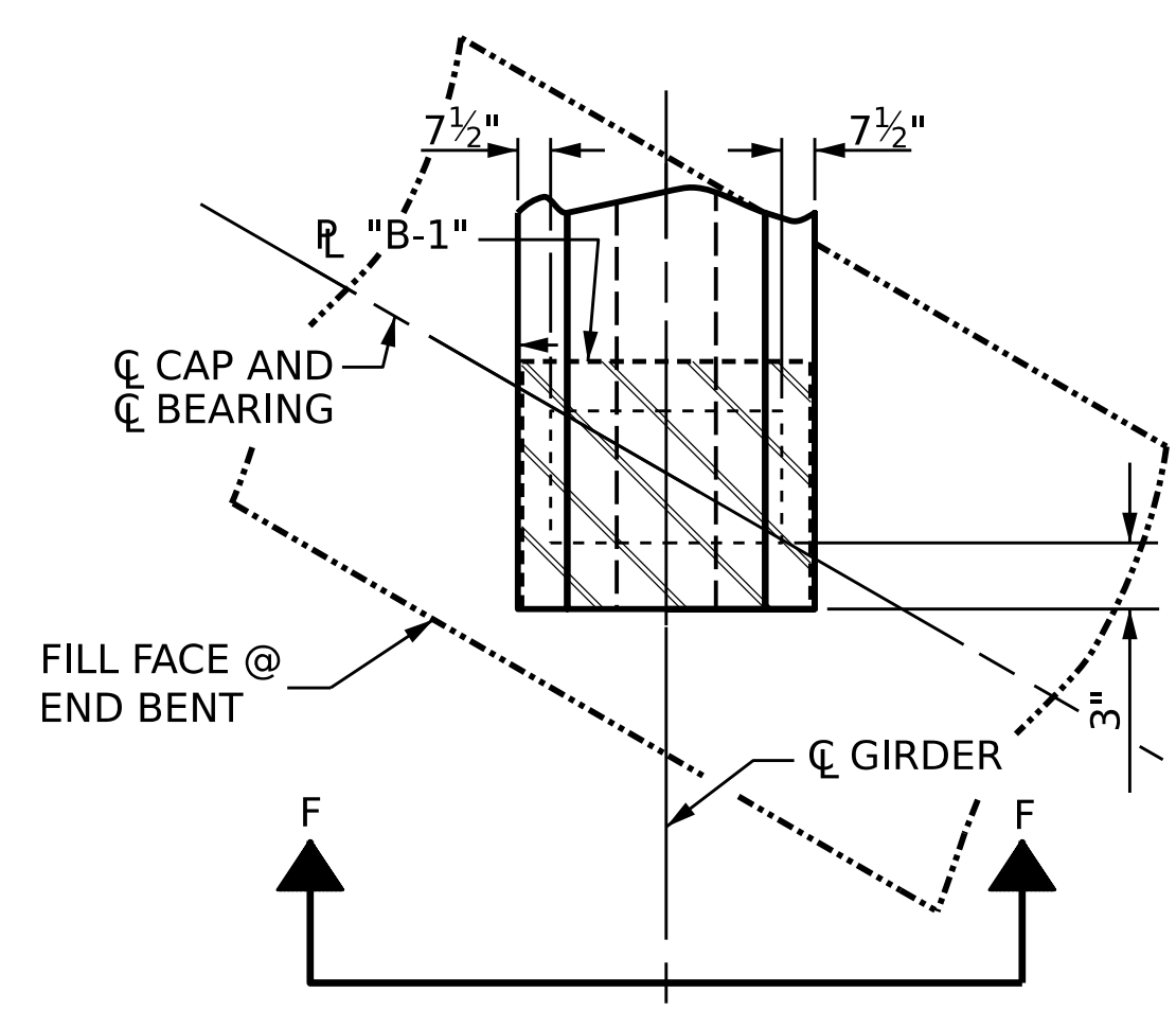
BEARING PLAN AT BENT
