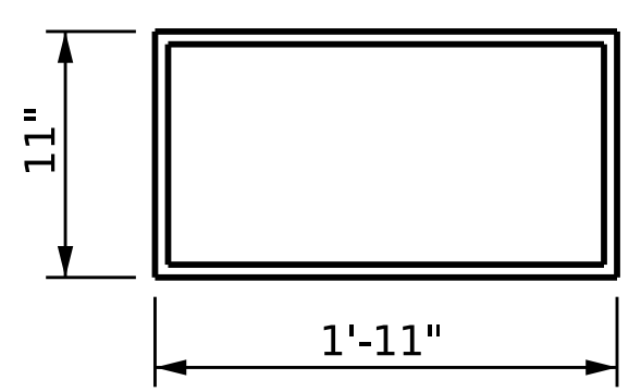
E1 (24 REQ'D) PLAN VIEW OF ELASTOMERIC BEARING
