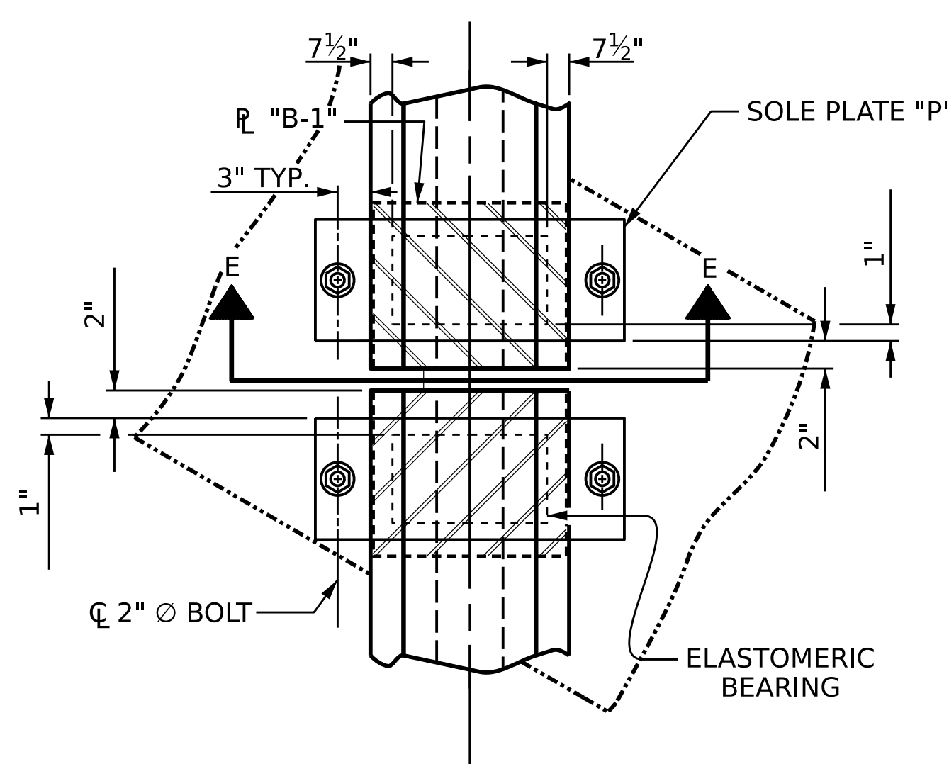
BEARING PLAN AT BENT
