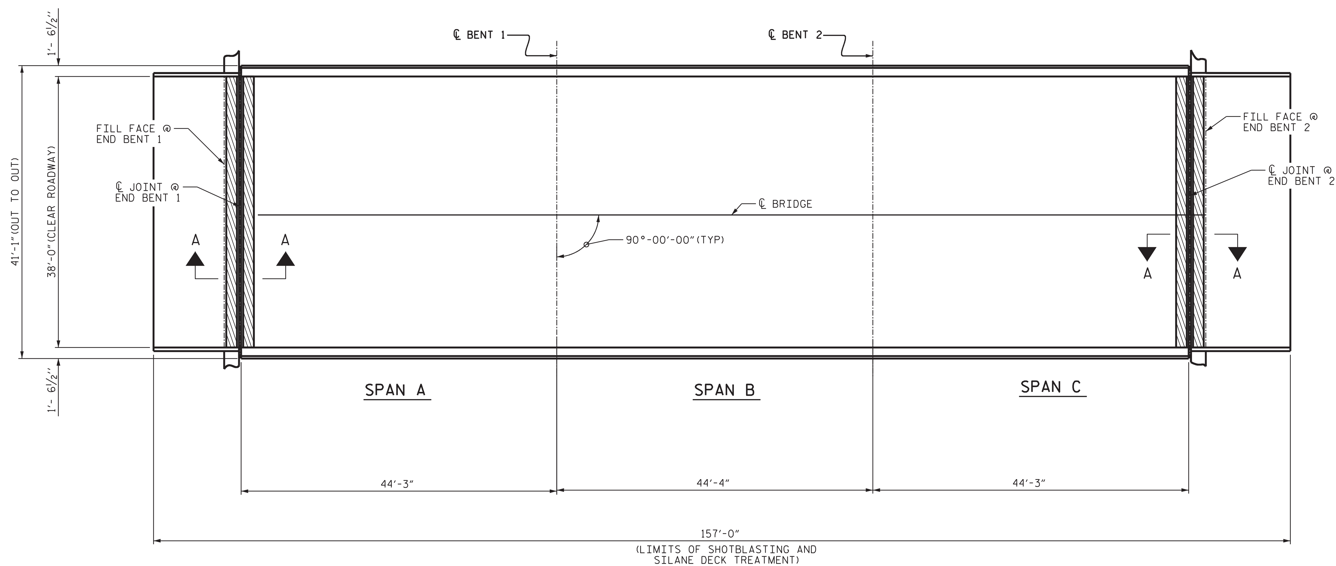
PLAN OF SPAN A-C
