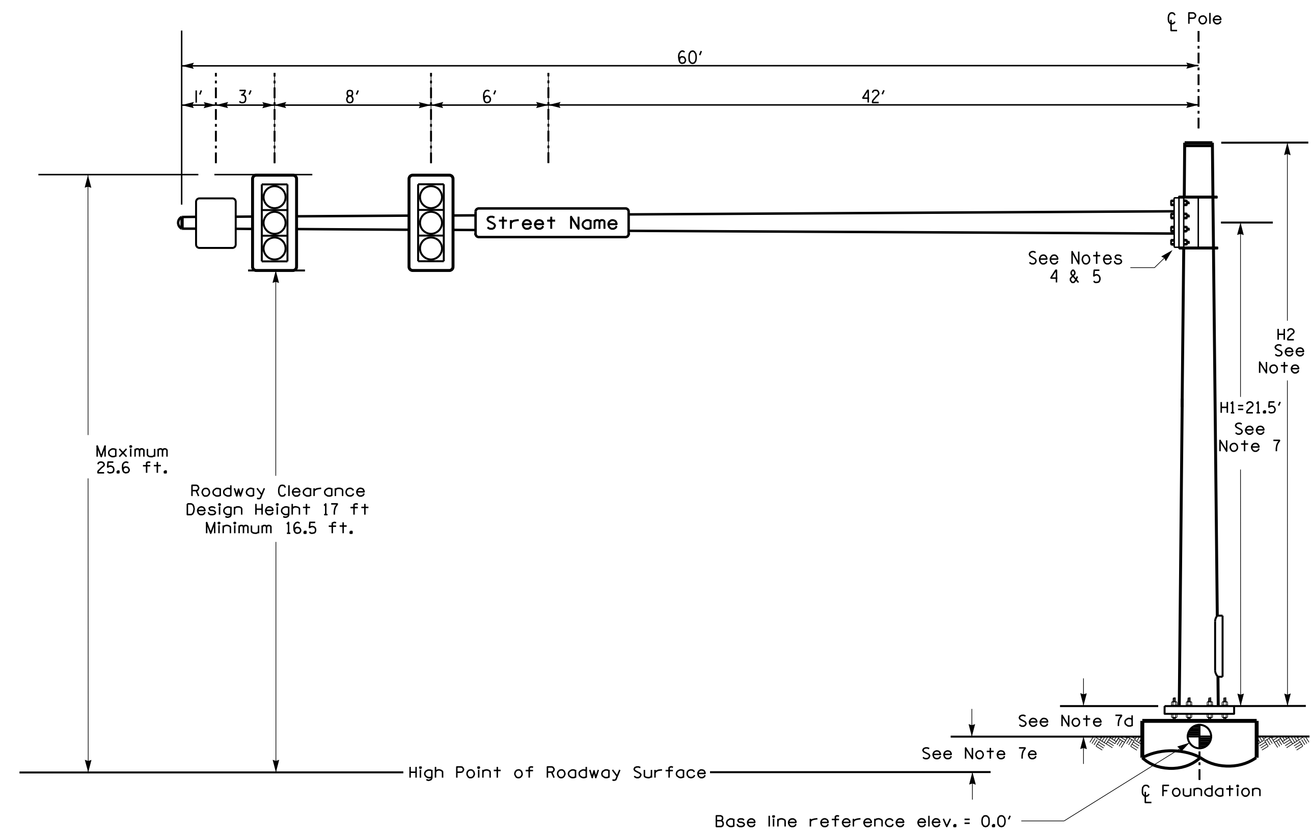
Elevation View
