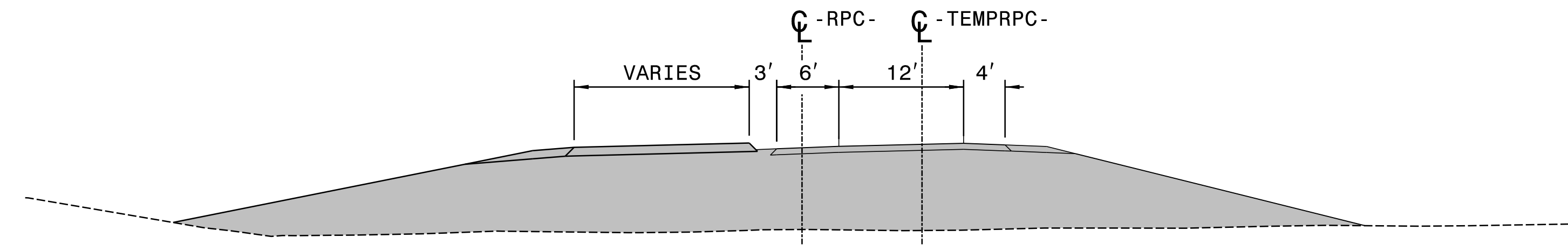
SECTION F-F
