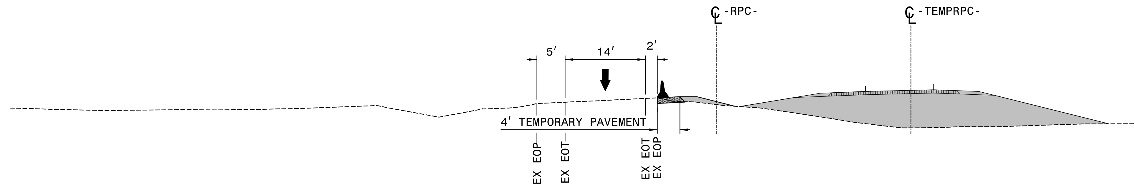
SECTION E-E
