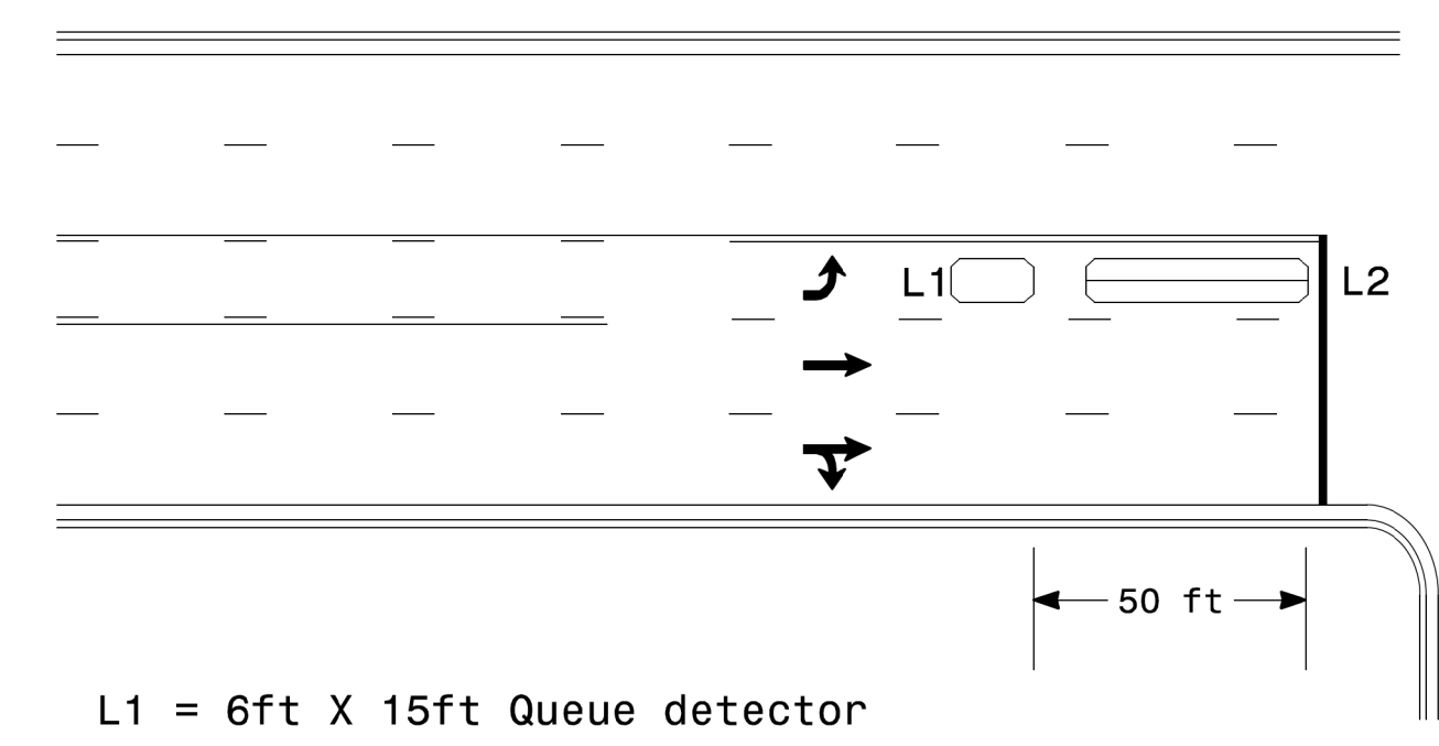
Queue Loop Detection
