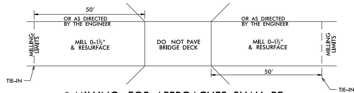
BRIDGE DRAWING FOR MAP #7 RAYS BRIDGE RD BRIDGE #132
