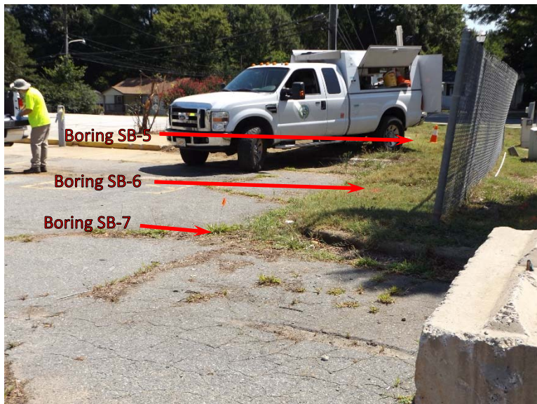
Photograph 8. GeoEnvironmental soil boring locations SB-5, SB-6, and SB-7.
